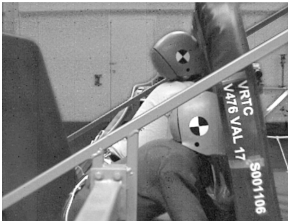
Figure 20. Lap Belt Test at Maximum Neck Extension, 150 msec
