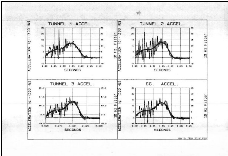
Figure 5. Longitudinal Deceleration Profiles at Different Locations on the Bus
