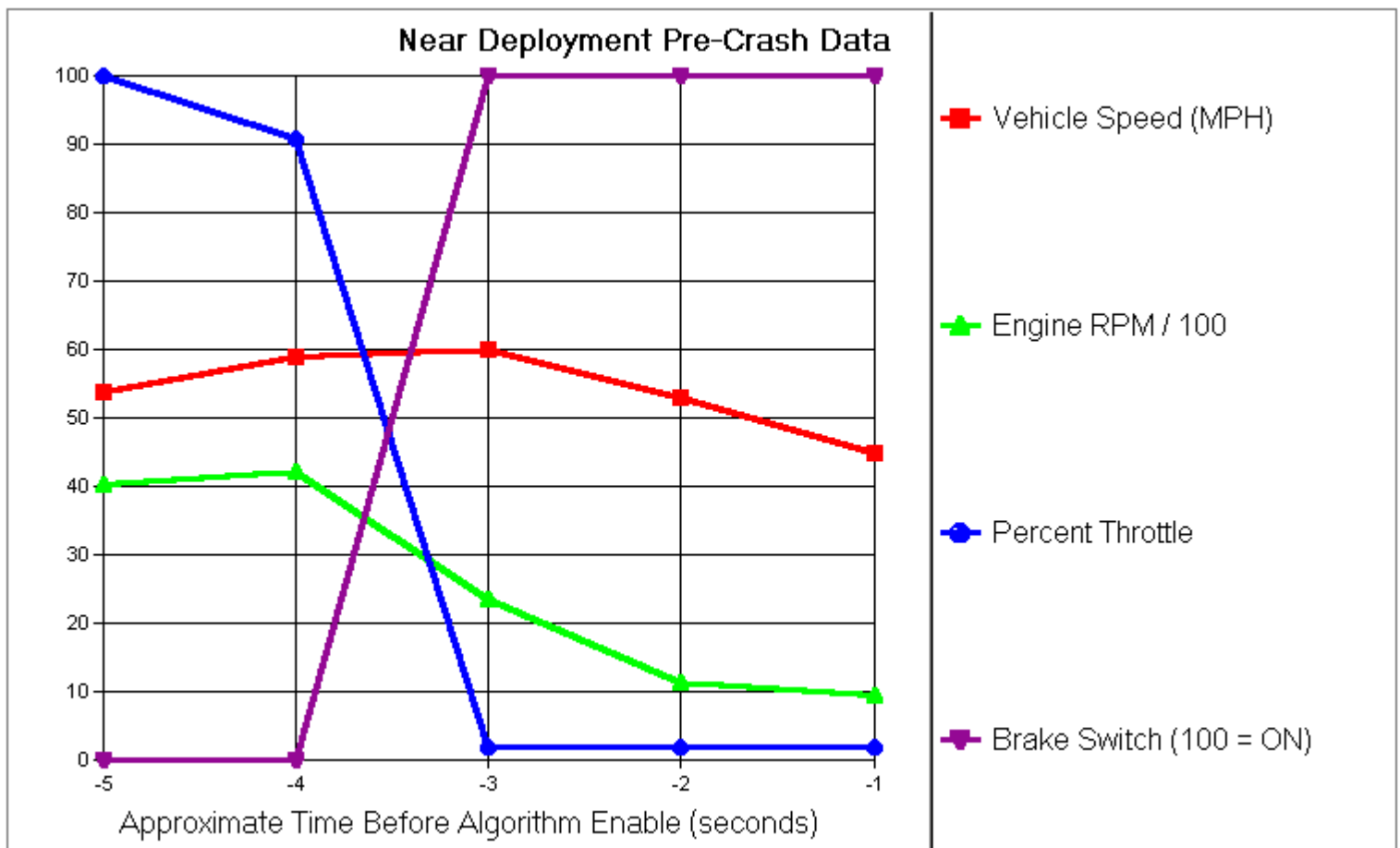
Figure 2. Chart of Pre-Crash Data
