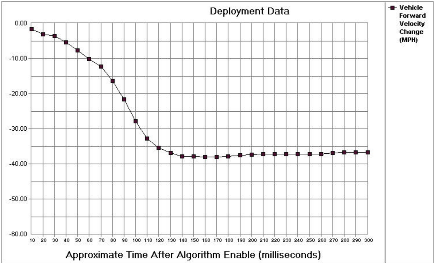
Figure 3. Chart of Delta-V versus Time
