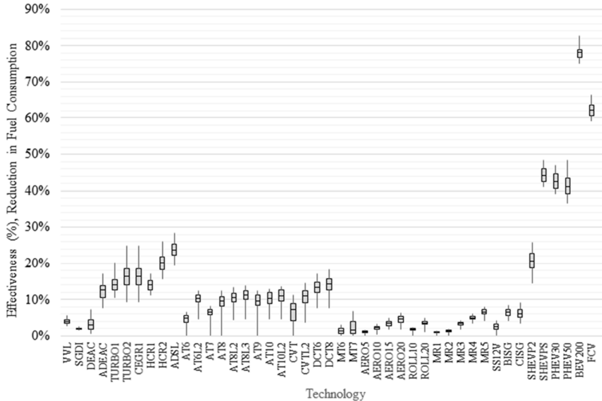
Technology Effectiveness Distribution (Includes all Technology Classes)
