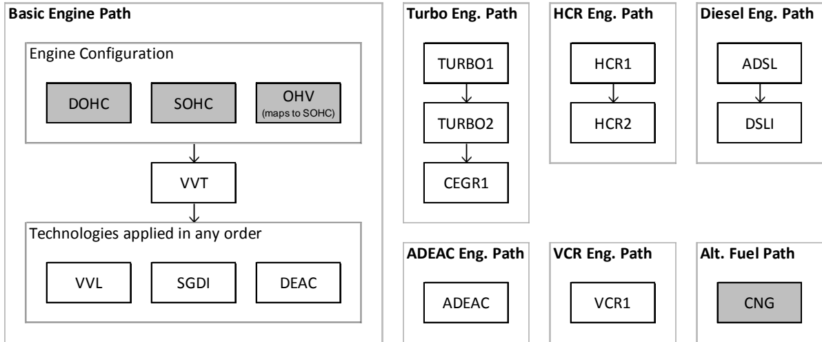
Figure-II-13 - Engine Paths
