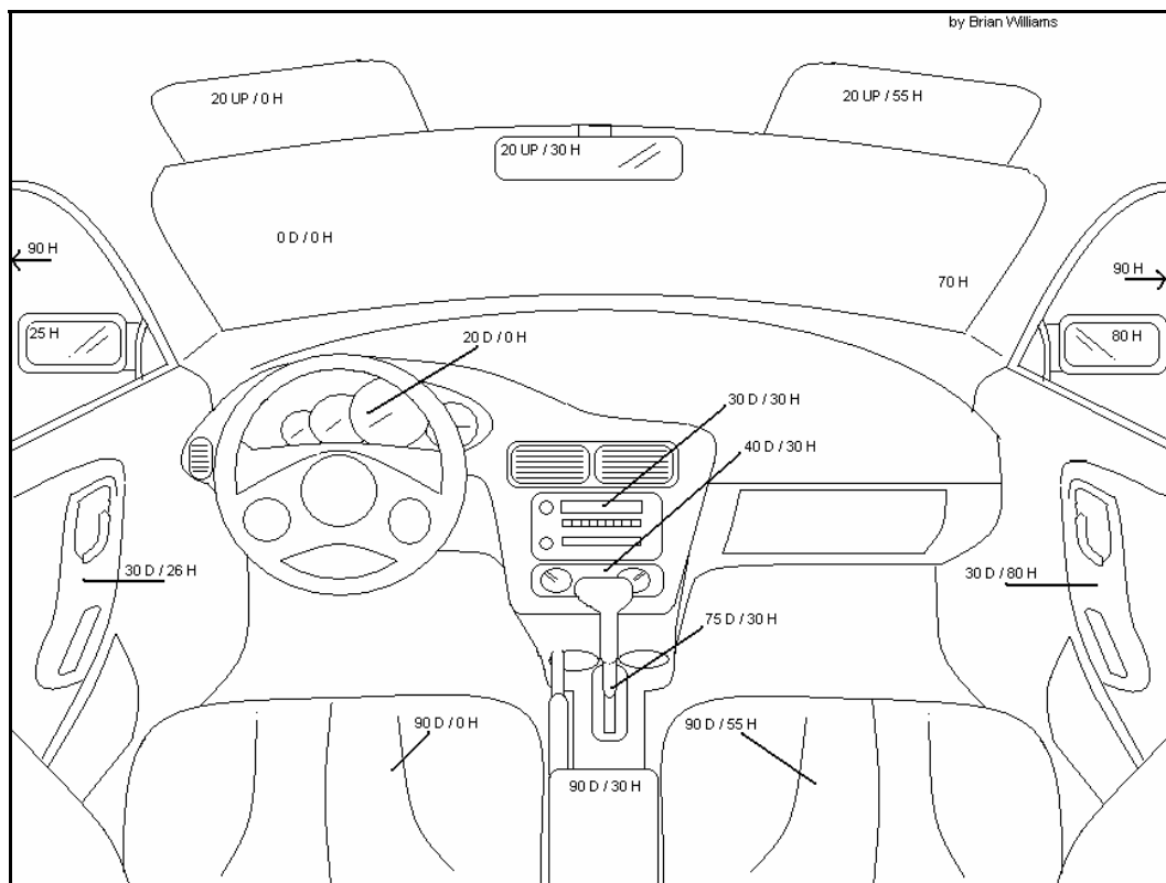
Figure 6.4. Depiction of degrees of visual angle from center forward that objects in the cockpit of an automobile are generally located.
