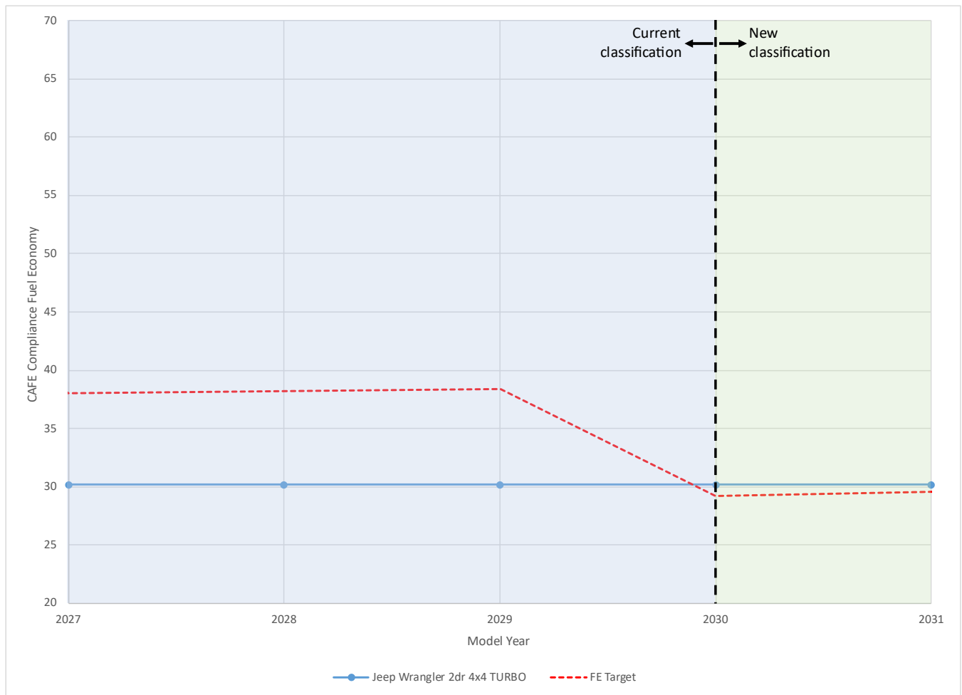
Figure 6-7: Jeep Wrangler 2dr 4x4 Turbo Compliance FE vs. CAFE Target FE
