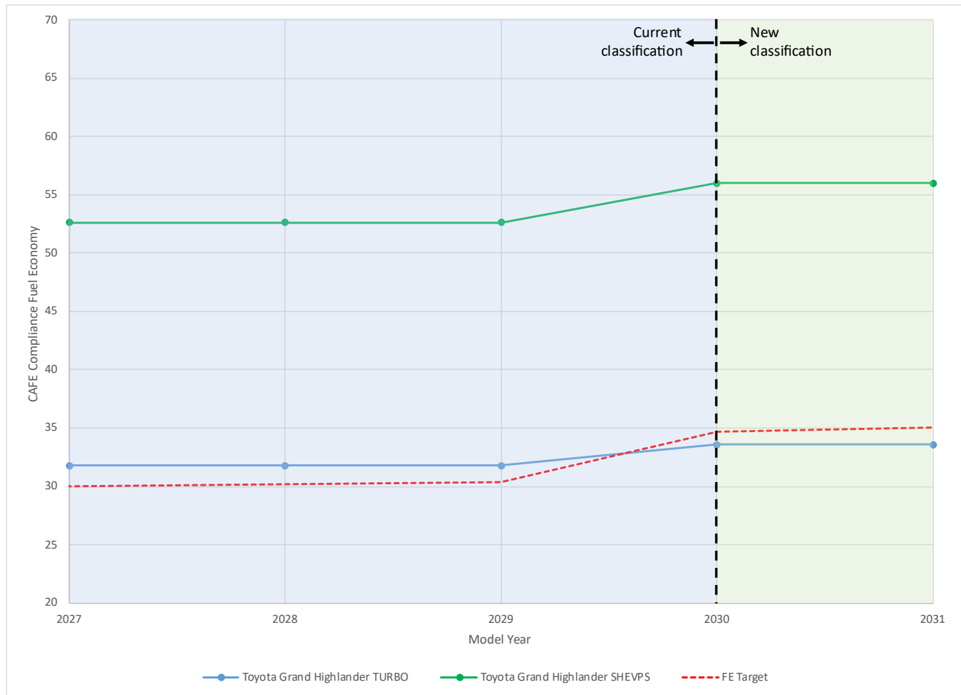
Figure 6-6: Toyota Grand Highlander All-Wheel Drive (AWD) Compliance FE vs. CAFE Target FE
