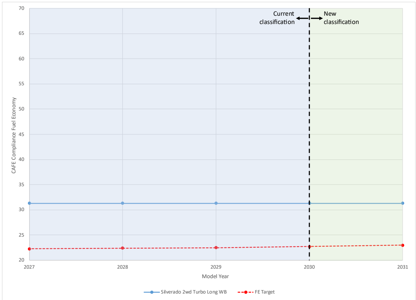
Figure 6-9: Chevrolet Silverado 2wd Turbo Compliance FE vs. CAFE Target FE
