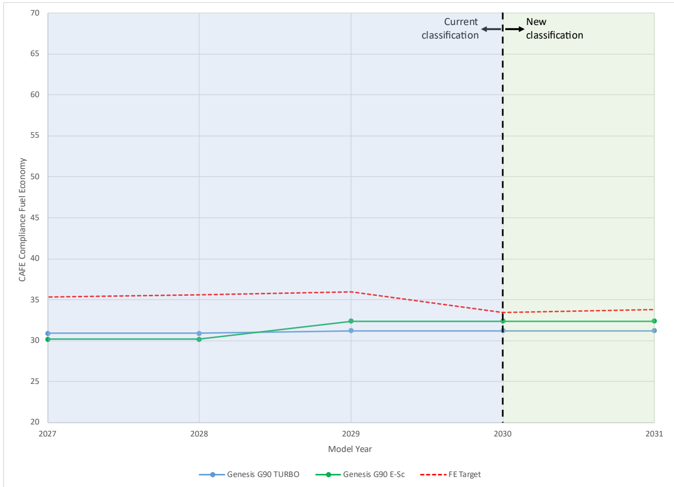
Figure 6-3: Genesis G90 3.5T AWD Compliance FE vs. CAFE Target FE
