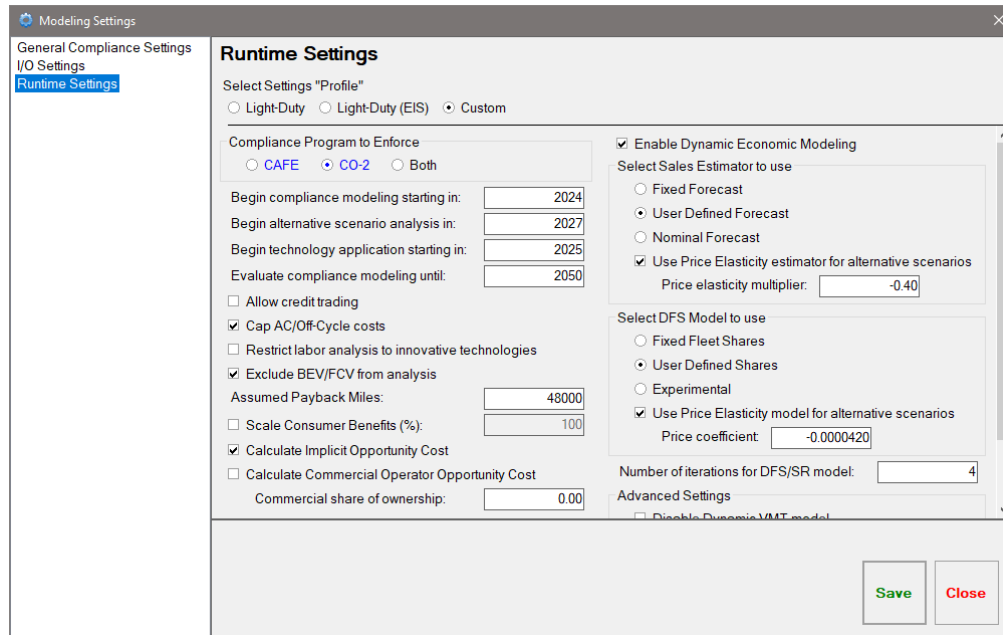
Figure 38. Enable Compliance with CO 2 Standards
