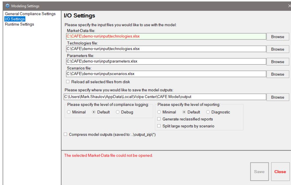
Figure 17. I/O Settings Panel (2)
