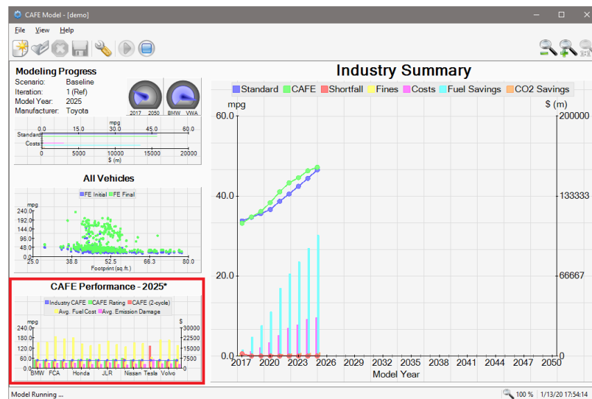
Figure 22. Session View - Compliance Performance Chart
