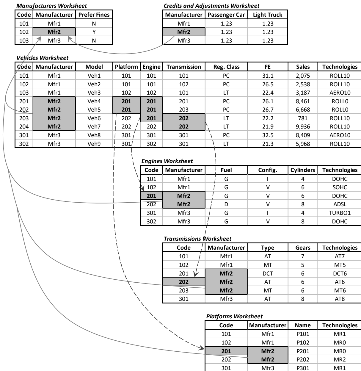
Figure 1. Basic Structure of Input File Defining the Fleet's Initial State 4
