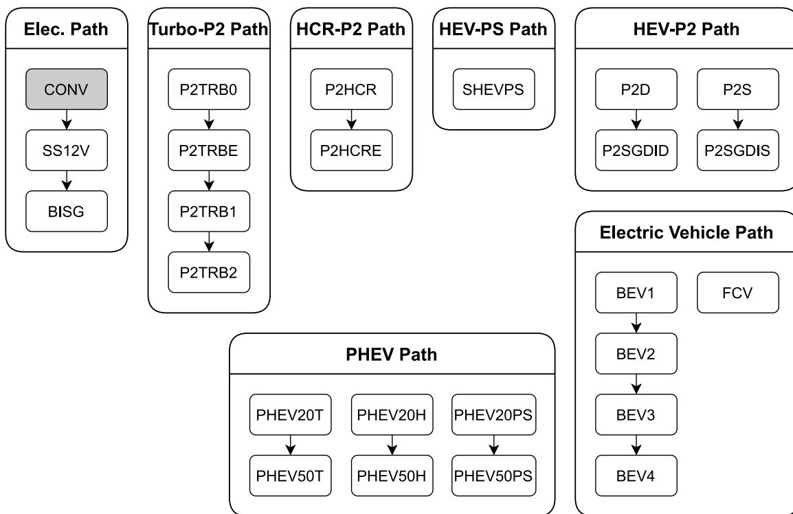
Figure 4. Vehicle-Level (Electrification & Hybrid/Electric) Paths
