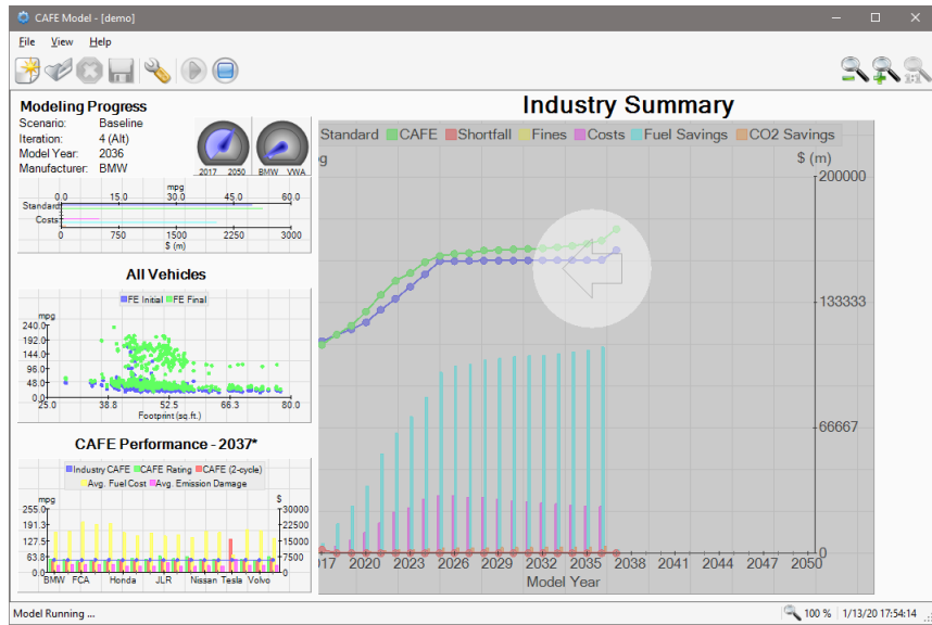
Figure 24. Initiating Chart Filtering
