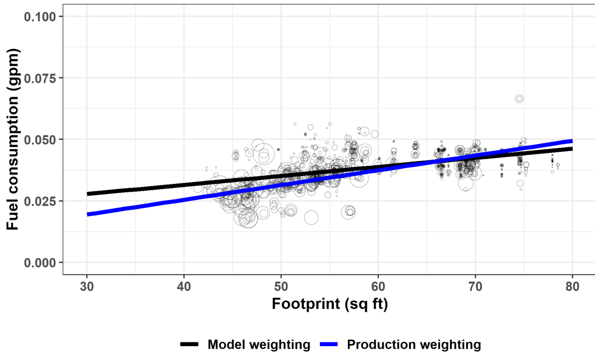
Figure 1-2: Footprint Curves via OLS by Weighting Scheme, MY 2022 Light Truck Fleet
