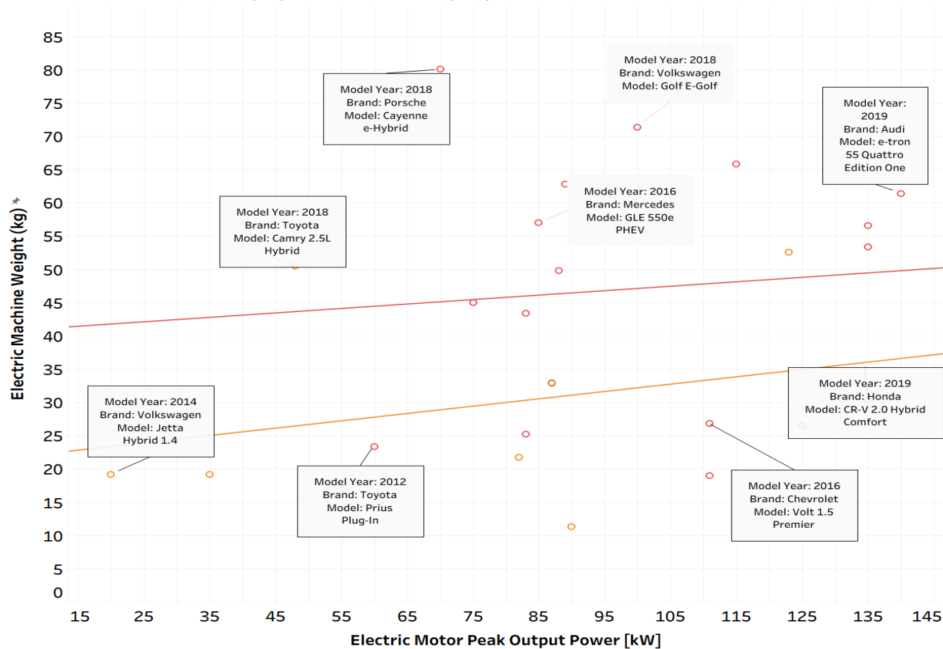
Figure 2-6: Electric Motor Mass Determination as Function of Peak Power
