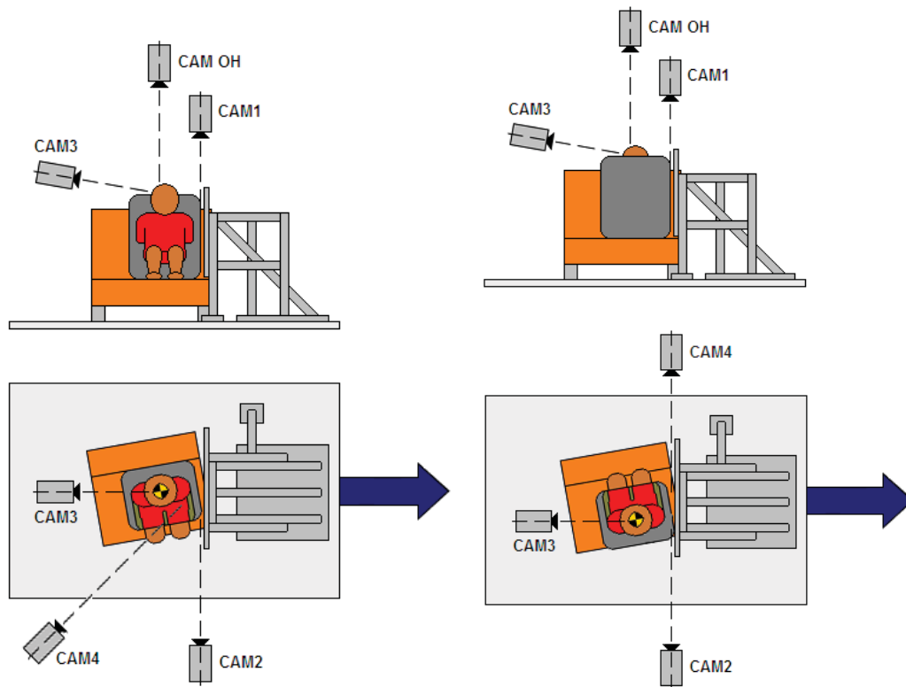
Figure 14: Camera positioning for forward facing CRS and rearward facing CRS tests
