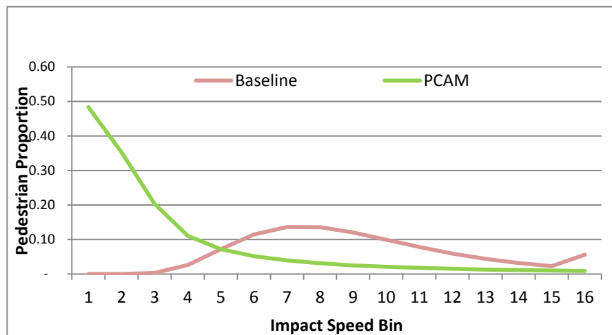
Figure 47. Smoothed Baseline and PCAM-Applicable Pedestrian Distribution for Weighted PCDS Cases for S3 Scenario, Pedestrian Walking, No Obstruction
