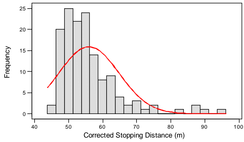
Figure 3.2 – Histogram of Corrected Stopping Distance Data
