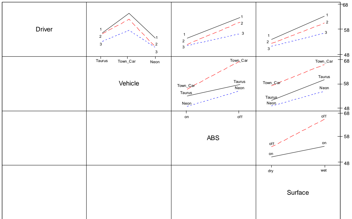
Figure 3.5 – Two-Way Interaction Plot of Corrected Stopping Distance Data
