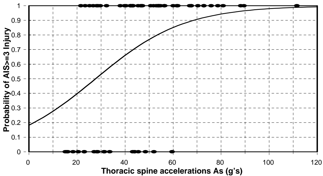
Figure 4-2. Probability of injury using spinal acceleration as risk factor (model I). Filled in circles represent 71 sled test data categorized as AIS \geq 3 injury (=1) and AIS < 3 injury (=0).
