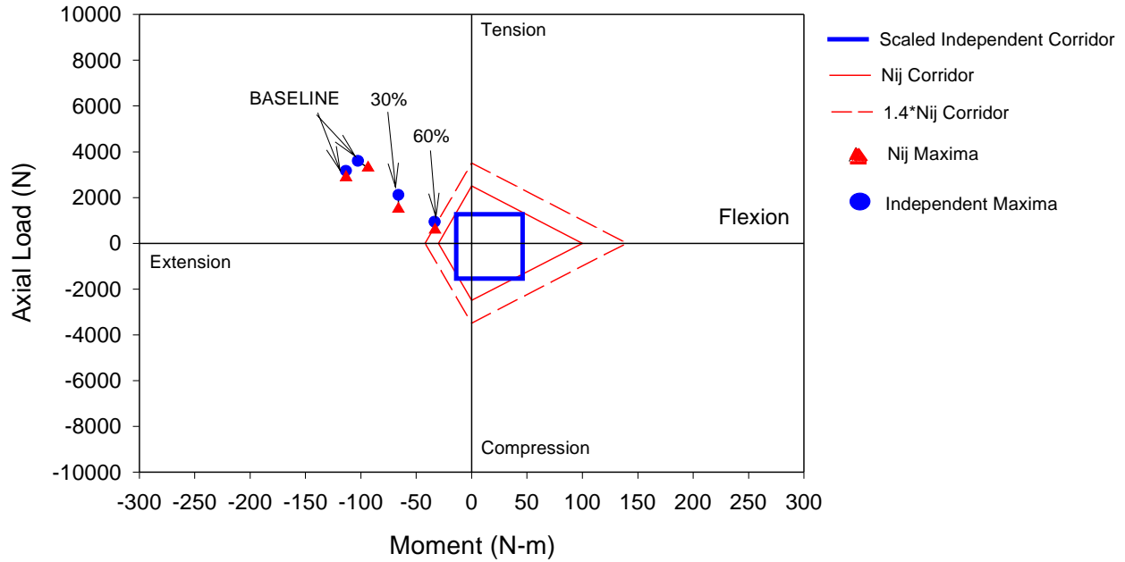
Figure A-23. Comparison of Neck Injury Criteria for Out-of-Position Tests with Hybrid III 3YO Dummy in ISO 2 Position using air bag system B, model year 1994. The labels indicate tests performed with the unmodified baseline system or with the inflator with 30 or 60 percent propellant removed.
