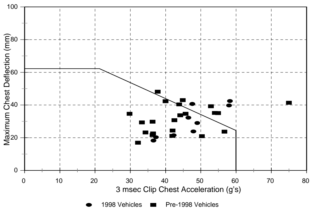
Figure B-7. 1998 and pre-1998 FMVSS208 Type Tests with the 5 th Percentile Female Hybrid III Belted Driver and Thoracic Injury Threshold Line for 5 th Percentile Female Dummy. The passing rate for the dummy in the driver position in these tests is 72%.
