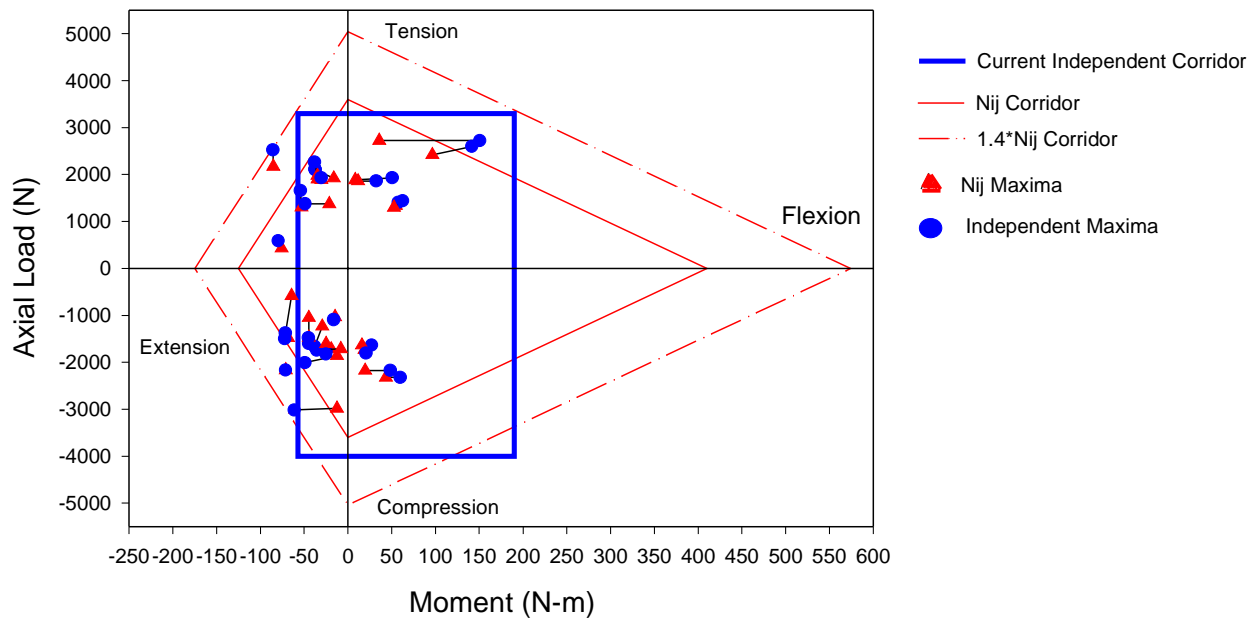
Figure A-4. Comparison of Neck Injury Criteria for 1997 NCAP Tests with ATD in Passenger Position.
