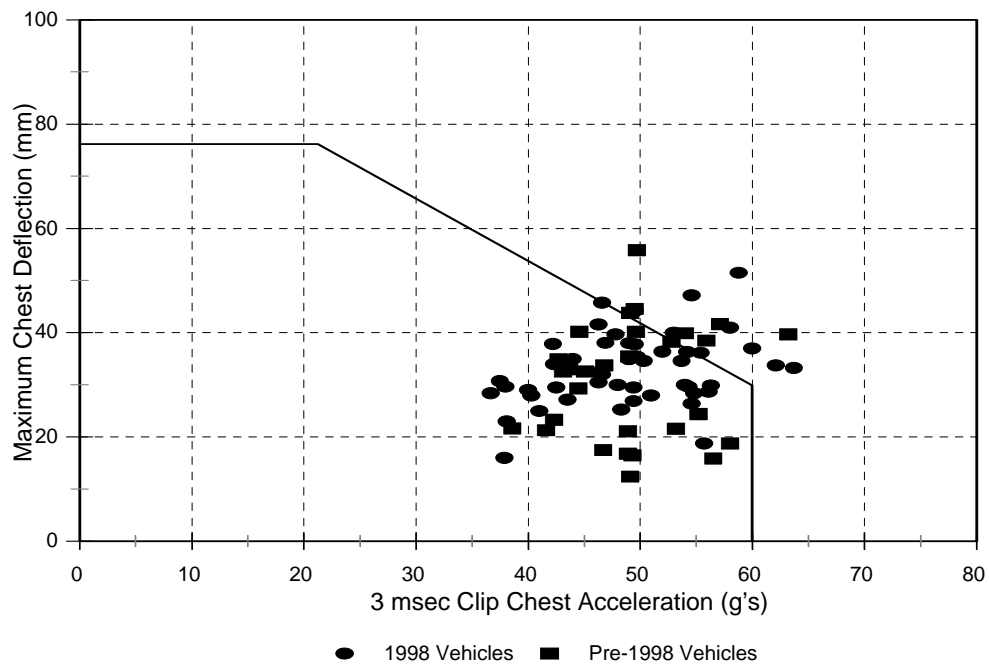
Figure B-2. 1997 and 1998 NCAP Crash Tests with the ATD in the Passenger Position and Thoracic Injury Threshold Line for 50 th Percentile Male Dummy. The passing rate for the dummy in the passenger position is 80%.
