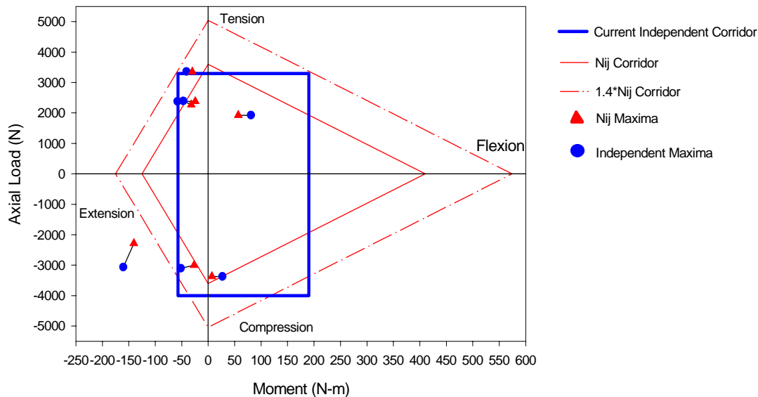
Figure 3-3. Typical Plot Comparing Nij with Current Injury Criteria.
