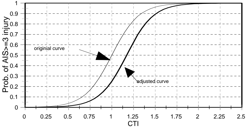
Figure 4-11. Reduced probability of injury using Model VII as the risk factor to relate sled test data to real world crashes. A value of one corresponds to 25% probability of injury.
