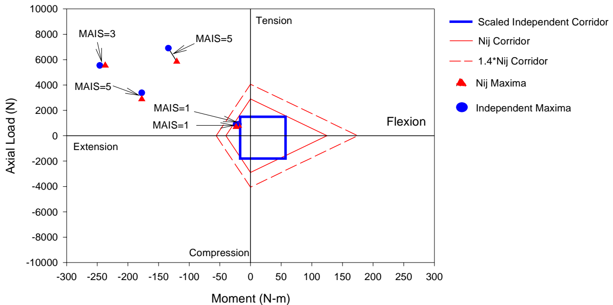
Figure A-28. Comparison of Neck Injury Criteria for Hybrid III 6YO Dummy Data from NASS and SCI Case Reconstructions.
