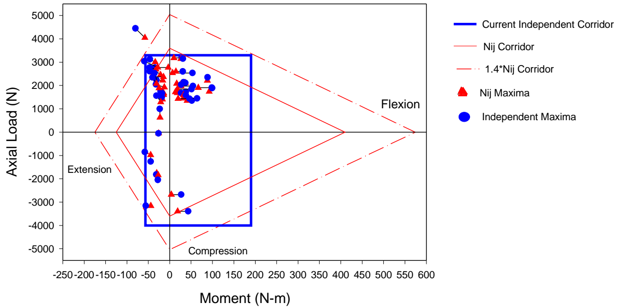
Figure A-1. Comparison of Neck Injury Criteria for 1998 NCAP Tests with ATD in Driver Position.
