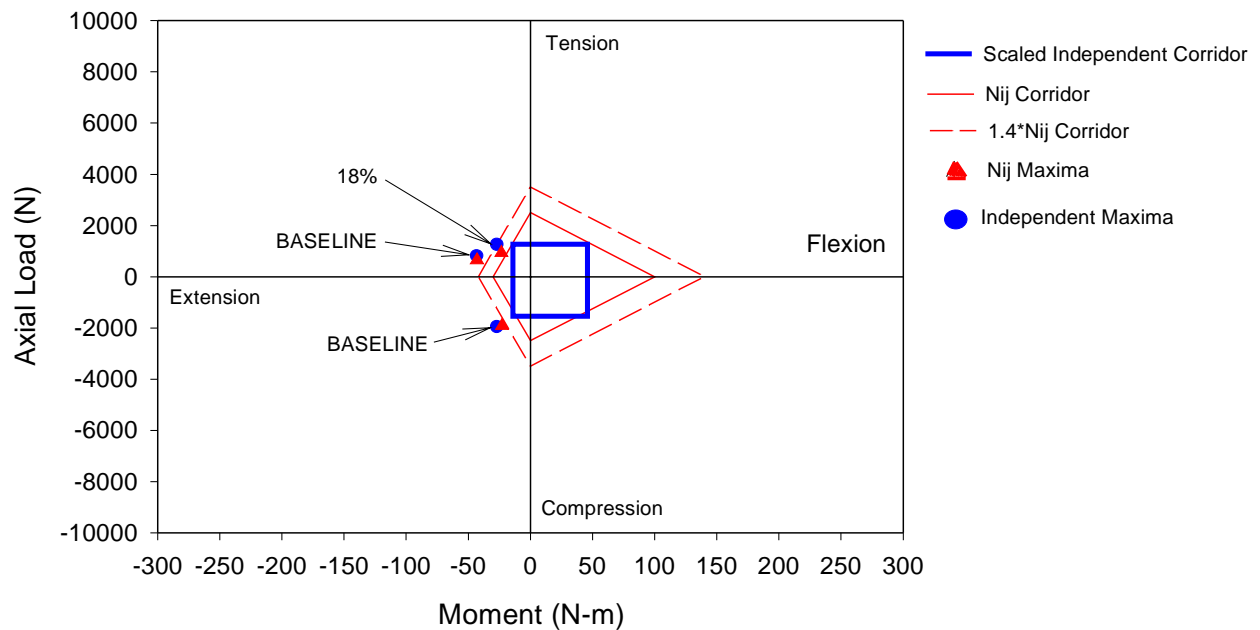
Figure A-25. Comparison of Neck Injury Criteria for Out-of-Position Tests with Hybrid III 3YO Dummy in ISO 2 Position using air bag system D, model year 1996. The labels indicate tests performed with the unmodified baseline system or with the inflator with 18 percent propellant removed.
