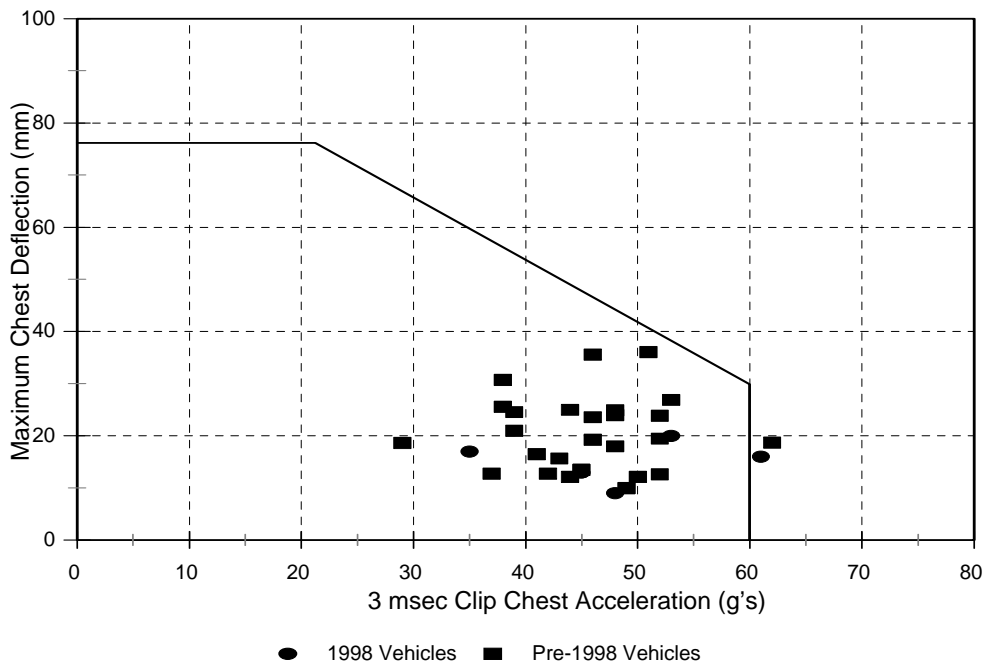
Figure B-4. 1996 -1998 FMVSS 208 Crash Tests with the ATD in the Passenger Position and Thoracic Injury Threshold Line for 50 th Percentile Male Dummy. The passing rate for the dummy in the passenger position is 94%.
