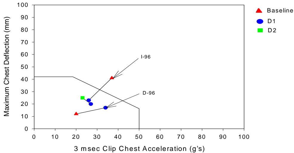
Figure B.13- ISO-1 out-of-position test data for 3-year old dummy with baseline and propellant removed air bags (D1 and D2). Tests using the same air bag module are connected by lines. The thoracic injury threshold line is for a 3 year old. The percentage of propellant removed in D2 is greater than in D1. As the propellant was removed, the aggressivity of the bag was reduced which produced lower thoracic injury values.
