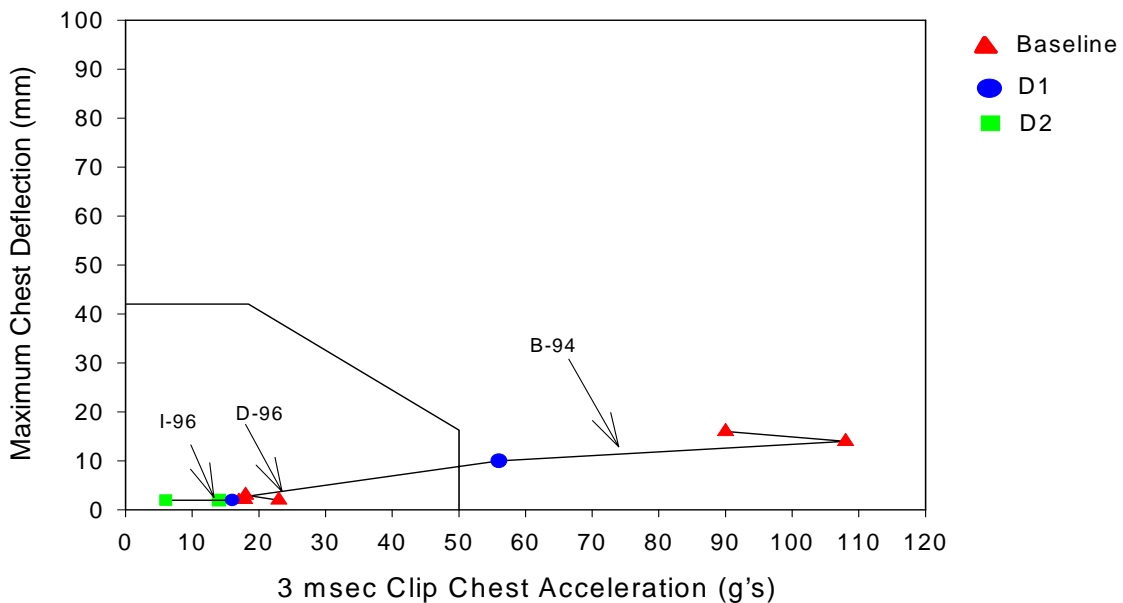
Figure B.14- ISO-2 out-of-position test data for 3-year old dummy with baseline and propellant removed air bags (D1 and D2). Tests using the same air bag module are connected by lines. CTI threshold line is for a 3 year old. The percentage of propellant removed in D2 is greater than in D1. As the propellant was removed, the aggressivity of the bag was reduced which produced lower thoracic injury values.
