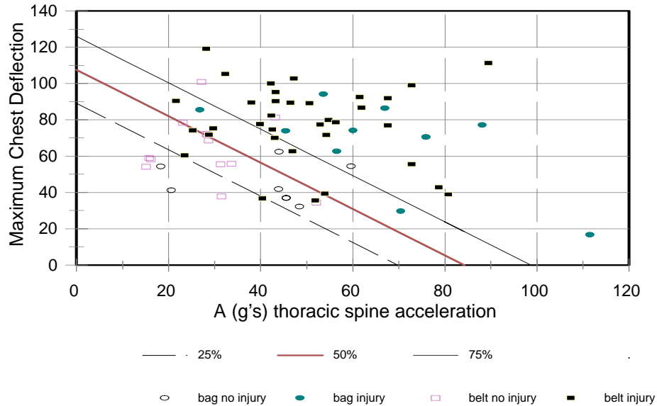
Figure 4-7. Lines of equal probability of AIS ≥3 injury using the linear combination of maximum deflection and spinal acceleration (Model VII). A 0 represents tests with AIS <3 and a 1 represents tests with AIS ≥1.
