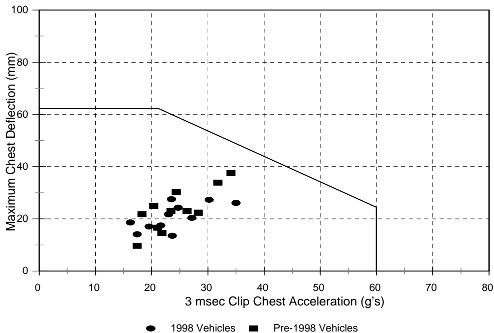
Figure B-5. 1998 and pre-1998 Vehicle Offset Crash Tests with the 5 th Percentile Female Hybrid III in the Driver Position and Thoracic Injury Threshold Line for 5 th Percentile Female Dummy. The passing rate for the dummy in the driver position is 100%.
