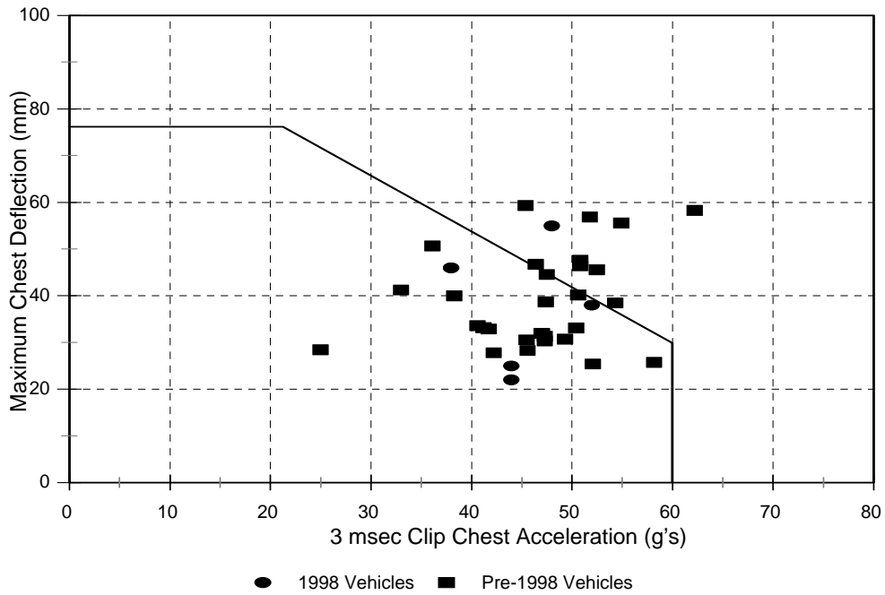
Figure B-3. 1996 - 1998 FMVSS 208 Crash Tests with the ATD in the Driver Position and Thoracic Injury Threshold Line for 50 th Percentile Male Dummy. The passing rate for the dummy in the driver position is 71%.
