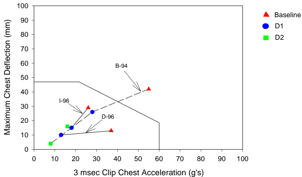
Figure B-11. ISO-1 out-of-position tests for 6 year-old dummy with baseline and propellant removed air bags (D1 and D2) and thoracic injury threshold lines for the 6 year-old dummy. Tests using the same air bag module are connected by lines. D2 has a greater percentage of propellant removed than in D1. As the propellant was removed, the aggressivity of the bag was reduced and produced lower thoracic injury values.
