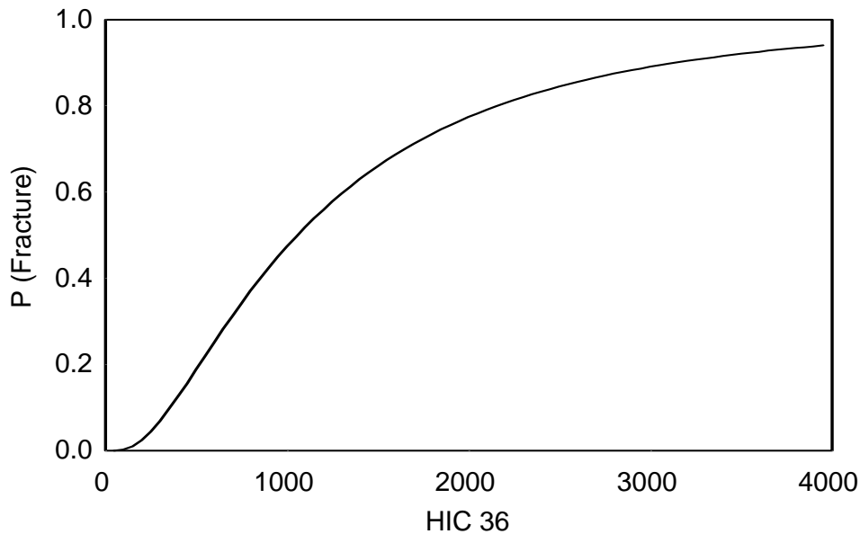
Figure 2-2. Injury risk curve for the Head Injury Criterion (HIC).
