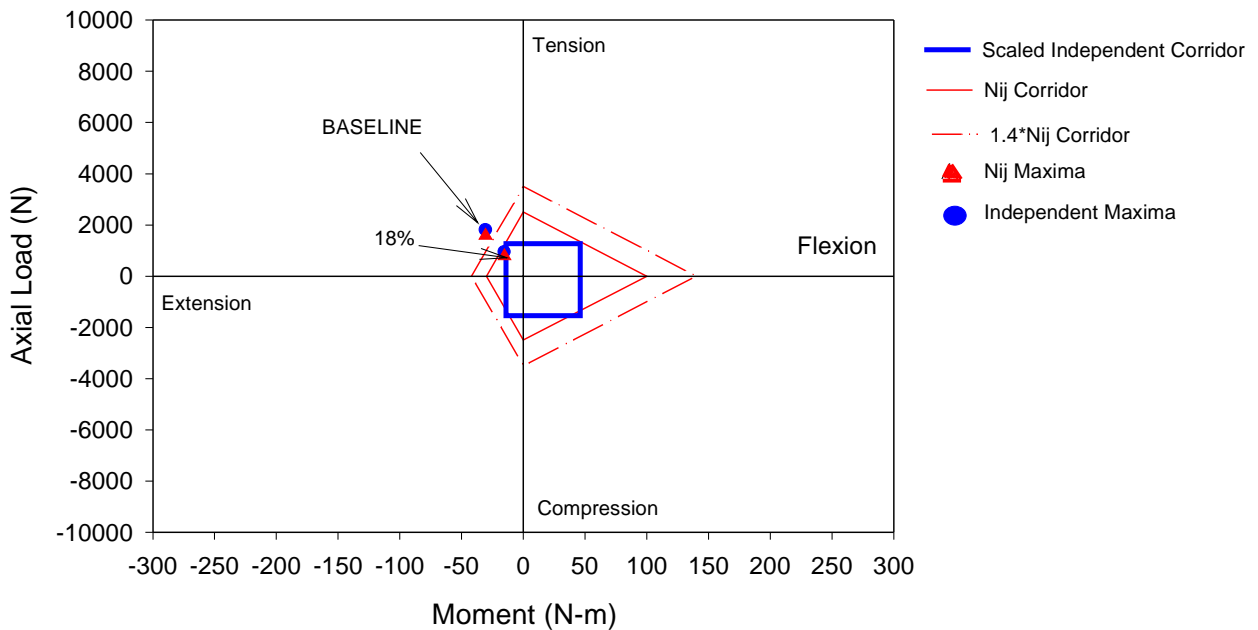
Figure A-24. Comparison of Neck Injury Criteria for Out-of-Position Tests with Hybrid III 3YO Dummy in ISO 1 Position using air bag system D, model year 1996. The labels indicate tests performed with the unmodified baseline system or with the inflator with 18 percent propellant removed.
