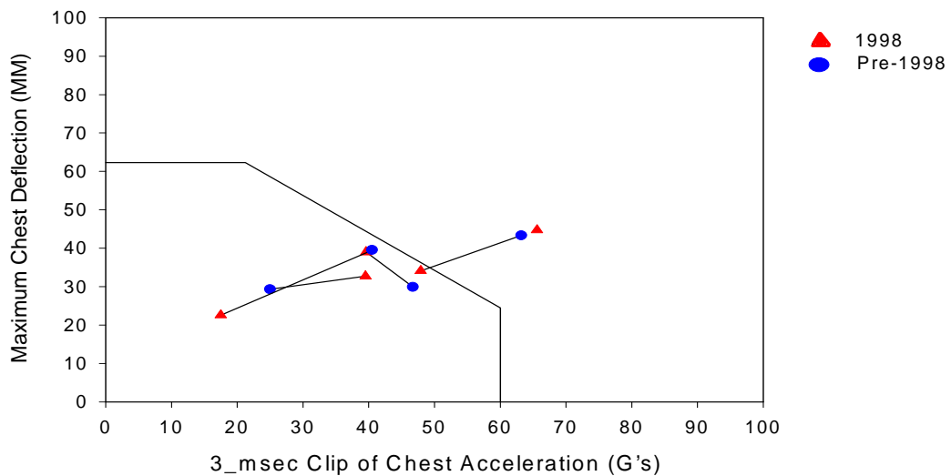
Figure B-10. 1998 and pre-1998 air bag systems with the 5 th percentile female dummy in the ISO-2 position and the corresponding thoracic injury threshold lines. Tests using the same air bag module are connected by lines. Not all 1998 vehicle air bags are less aggressive than their corresponding pre-1998 vehicle air bags in the ISO-2 condition.
