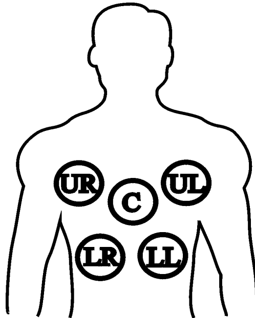
Figure 4-1. Location of five chest deflection measurement sites.
