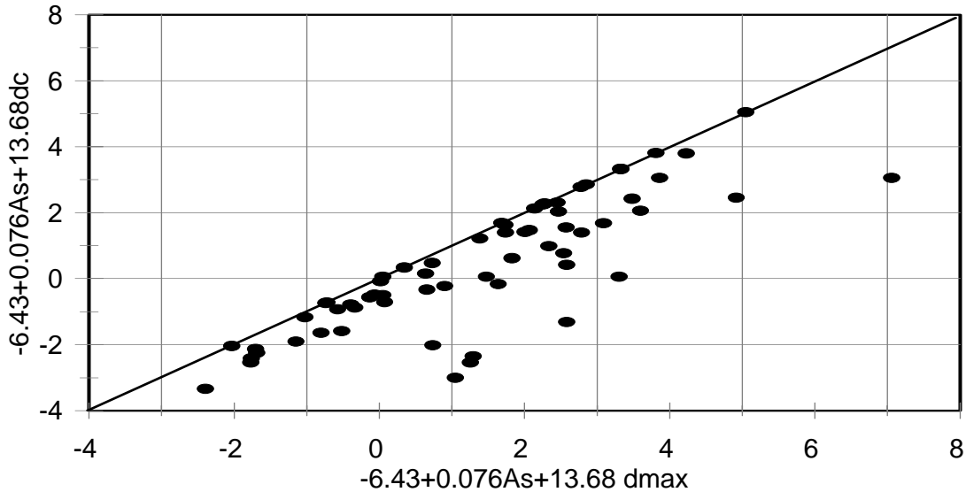
Figure 4-6. Model VII using dmax versus Model VII using dc as an estimator of dmax. The large differences in dmax and dc noted in Figure 4-5 is diminished due to the effect of spinal acceleration.
