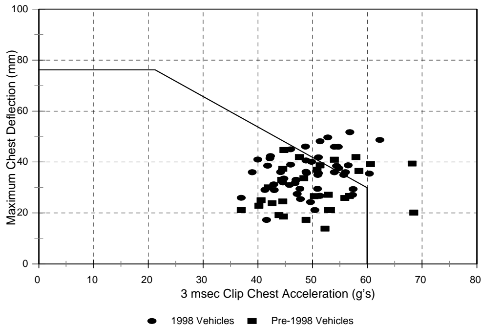
Figure B-1. 1997 and 1998 NCAP Crash Tests with the ATD in the Driver Position and Thoracic Injury Threshold Line for 50 th Percentile Male Dummy. The passing rate for the dummy in the driver position is 76%.
