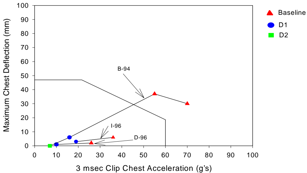
Figure B.12- ISO-2 out-of-position test data for 6-year old dummy with baseline and propellant removed air bags (D1 and D2). Tests using the same air bag module are connected by lines. The percentage of propellant removed in D2 is greater than in D1. As the propellant was removed, the aggressivity of the bag was reduced which produced lower thoracic injury values.
