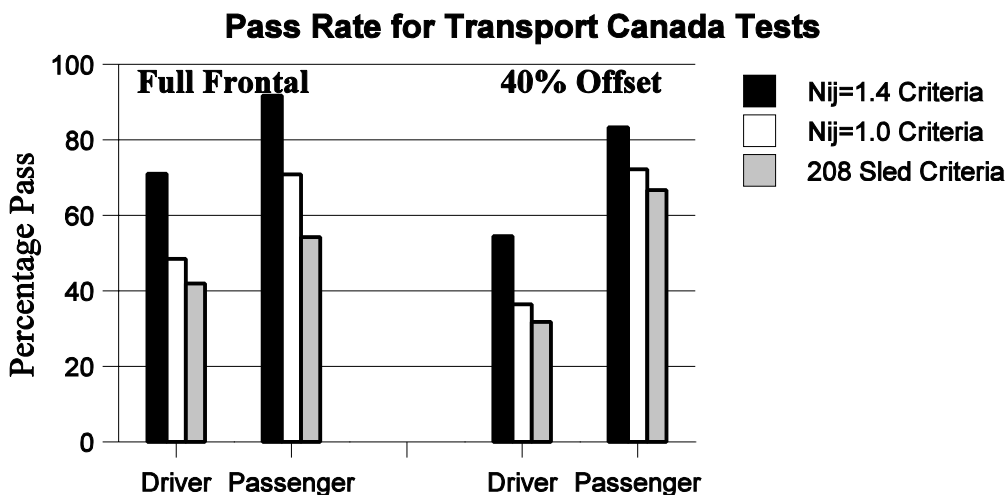
Figure 3-4. Comparison of Nij and Scaled 208 Criteria for Transport Canada Test Data.
