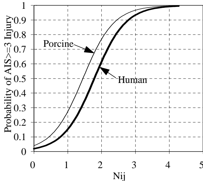
Figure 3-1. Injury Risk Curve for N ij Neck Injury Criteria.
