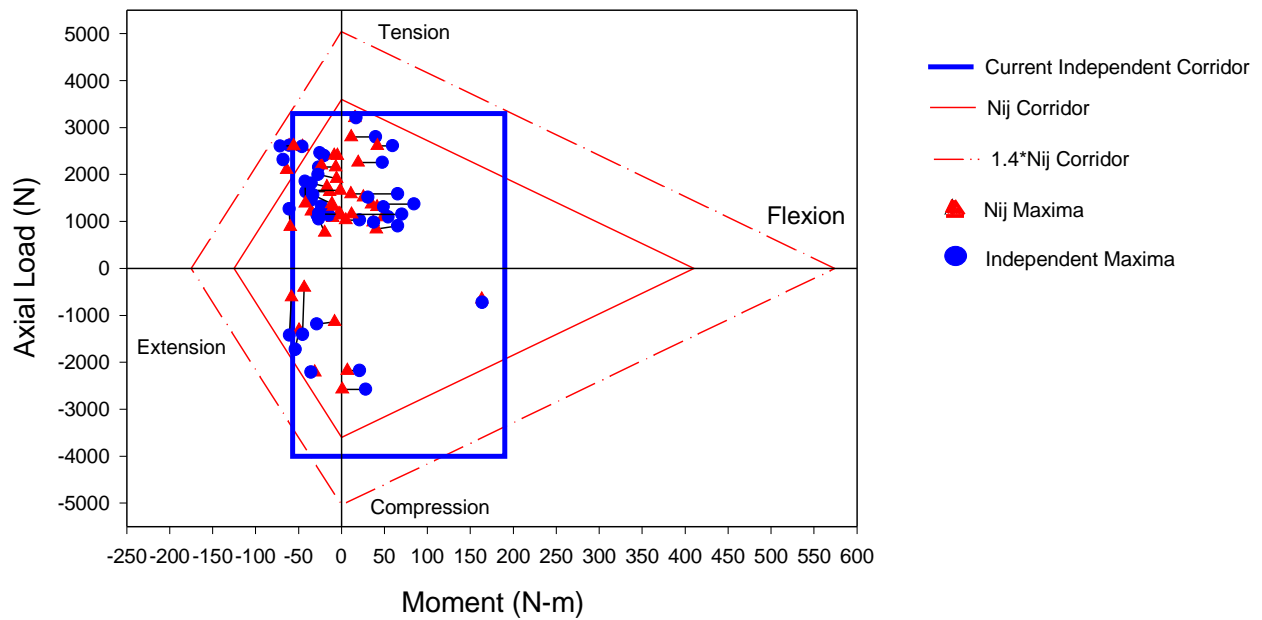
Figure A-2. Comparison of Neck Injury Criteria for 1998 NCAP Tests with ATD in the Passenger Position.
