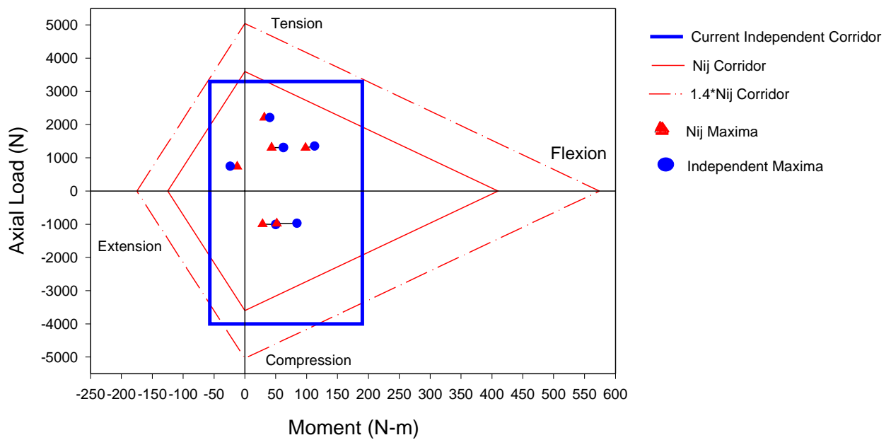
Figure A-6. Comparison of Neck Injury Criteria for 30 mph Unbelted Barrier Crash Tests for Vehicles using ATD in the Passenger Position.
