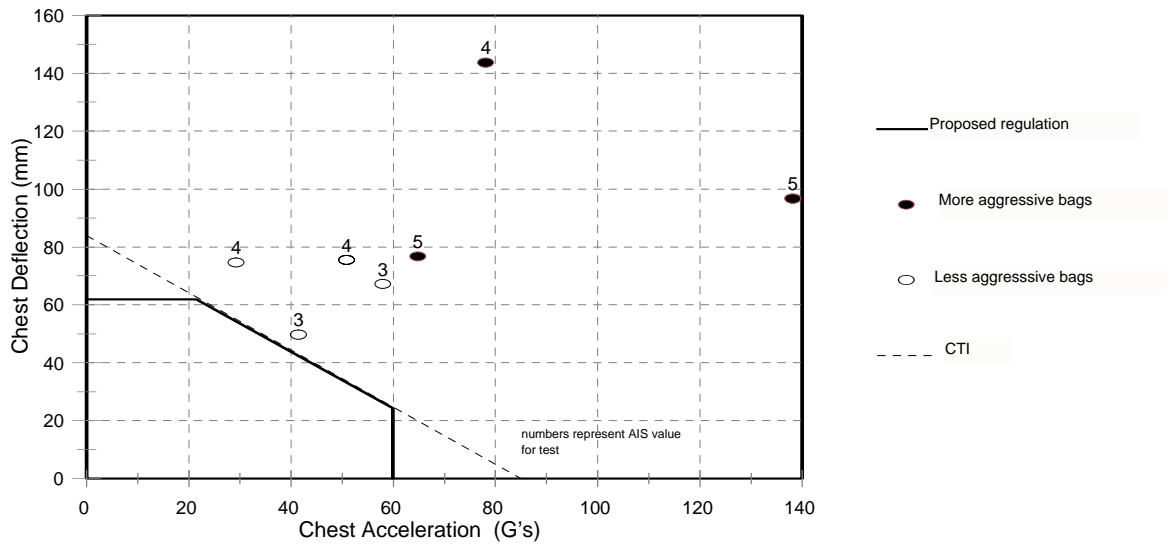
Figure 4-13. Proposed thoracic injury criteria for small female dummy and human surrogate ISO-2 OOP test data. Injury outcome in all the tests were AIS \geq 3 and all failed the proposed criteria.
