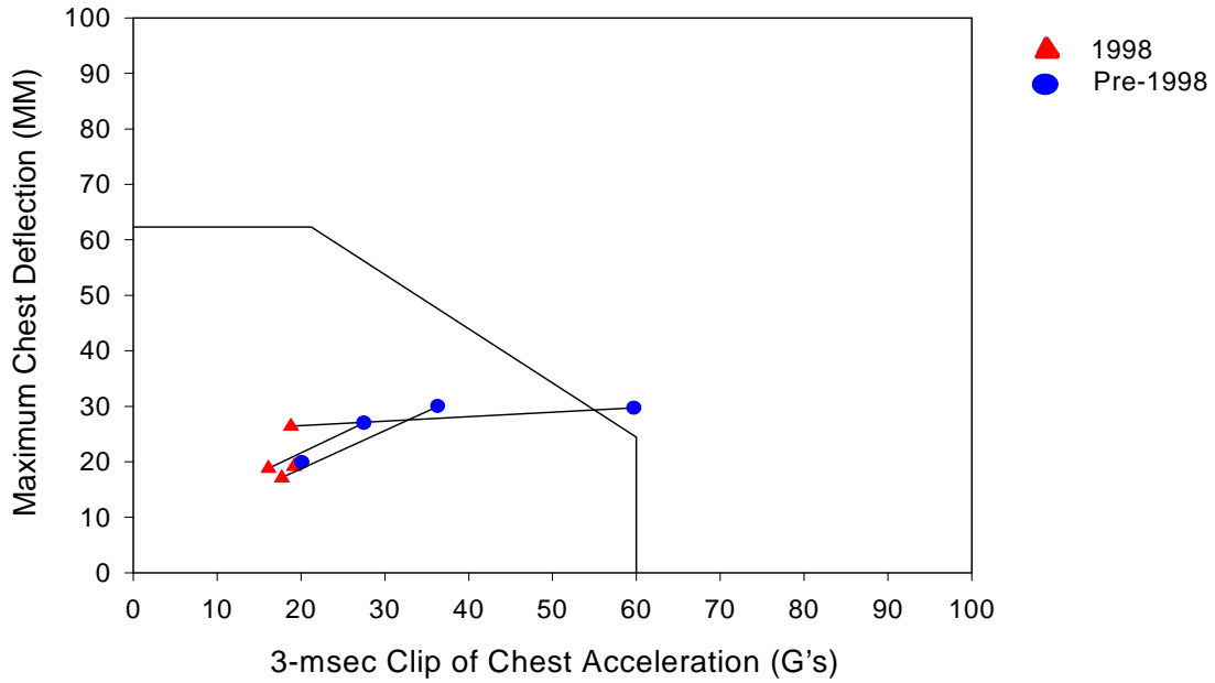
Figure B-9. 1998 and pre-1998 air bag systems with the 5 th percentile female dummy in the ISO-1 position and the corresponding thoracic injury threshold lines. Tests using the same air bag module are connected by lines. Only one pre-1998 vehicle air bag fails the thoracic injury criteria.
