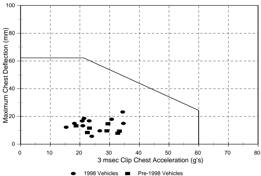
Figure B-6. 1998 and pre-1998 Vehicle Offset Crash Tests with the 5 th Percentile Female Hybrid III in the Passenger Position and Thoracic Injury Threshold Line for 5 th Percentile Female Dummy. The passing rate for the dummy in the driver position is 100%.
