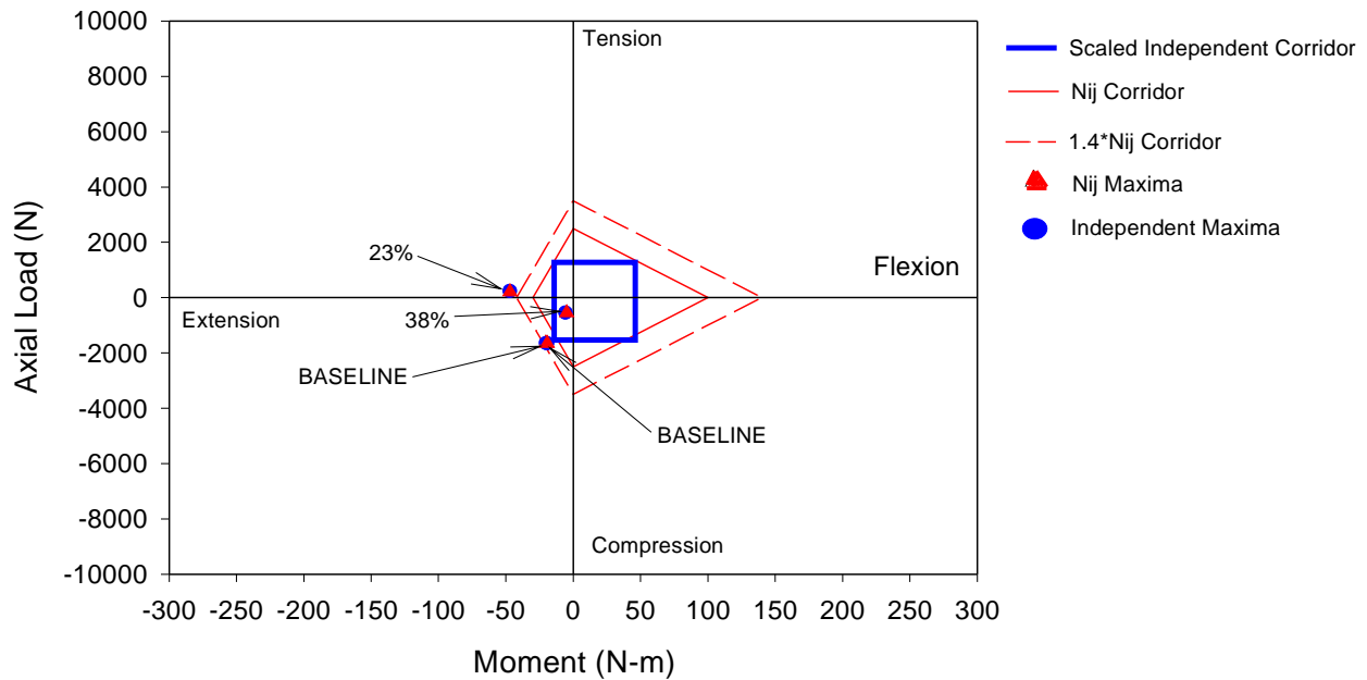
Figure A-27. Comparison of Neck Injury Criteria for Out-of-Position Tests with Hybrid III 3YO Dummy in ISO 2 Position using air bag system I, model year 1996. The labels indicate tests performed with the unmodified baseline system or with the inflator with 23 and 38 percent propellant removed.
