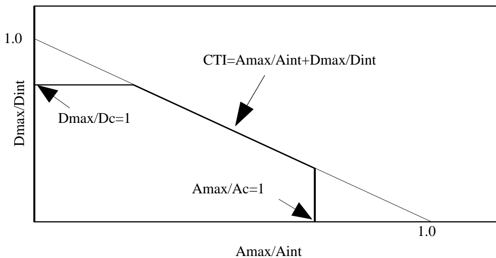
Figure 4-9. Normalized proposed injury criteria requirements for all dummy sizes.
