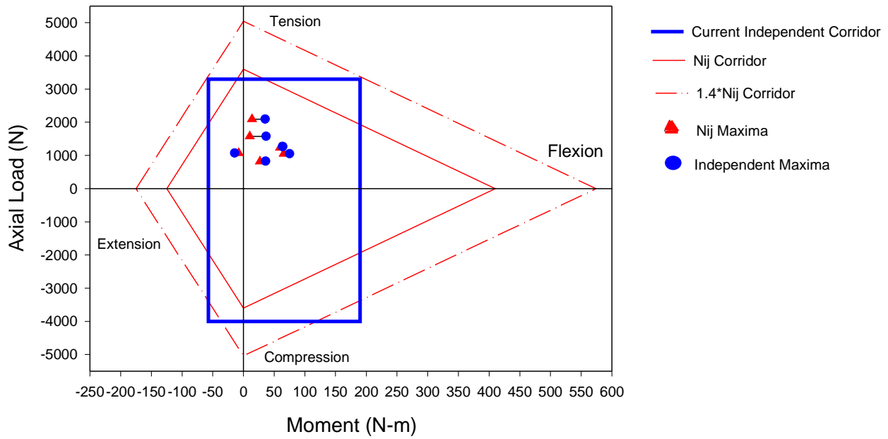
Figure A-5. Comparison of Neck Injury Criteria for 30 mph Unbelted Barrier Crash Tests for Vehicles using ATD in the Driver Position.
