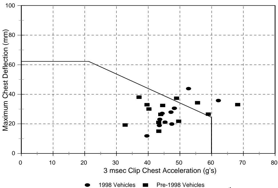
Figure B-8. 1998 and pre-1998 FMVSS208 Type Tests with the 5 th Percentile Female Hybrid III Belted Passenger and Thoracic Injury Threshold Line for 5 th Percentile Female Dummy. The passing rate for the dummy in the passenger position in these tests is 71%.
