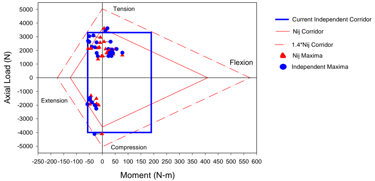
Figure A-3. Comparison of Neck Injury Criteria for 1997 NCAP Tests with ATD in the Driver Position.
