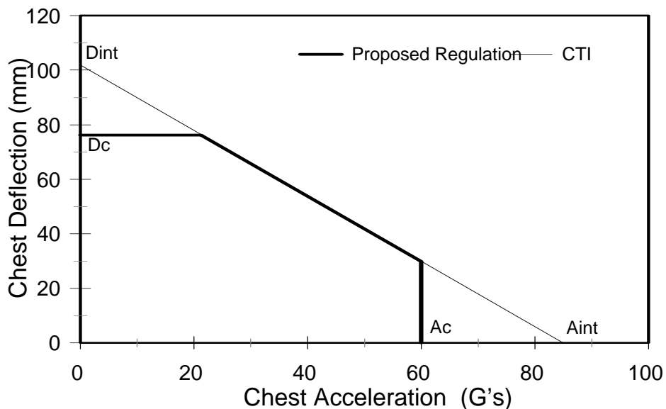
Figure 4-8. Injury criteria requirements for mid-sized adult male Hybrid III dummy.
