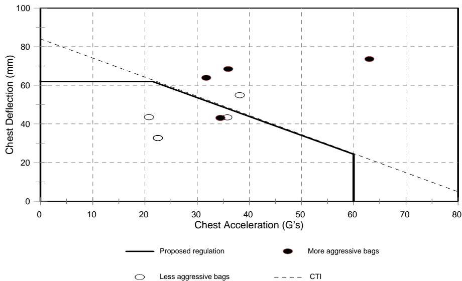
Figure 4-14. Proposed thoracic injury criteria for small female and ISO-2 OOP dummy tests. Most less aggressive airbags pass criteria while aggressive air bags fail the criteria.
