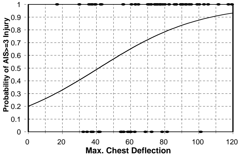
Figure 4-3. Probability of injury using maximum chest deflection ( d_{max} ) as risk factor (model III).
