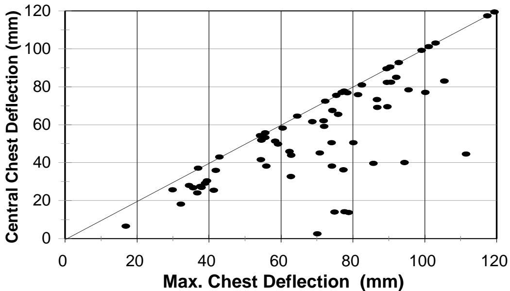
Figure 4-5. Plot of d_{max} versus d_c . Maximum chest deflection occurs at the central chest location in only 25% of the tests.
