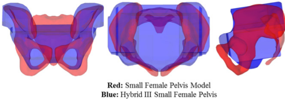
Figure 3b. Comparison of SFPM geometry and Hybrid III geometry aligned to hip joint centers.
