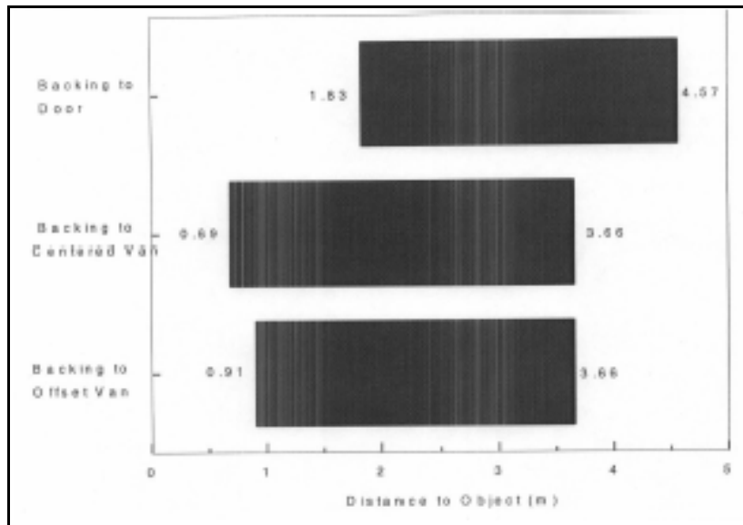
Figure 1 Shortest and Longest Detection Zones to Cardboard Target Covered by Rear Object Detection Systems
