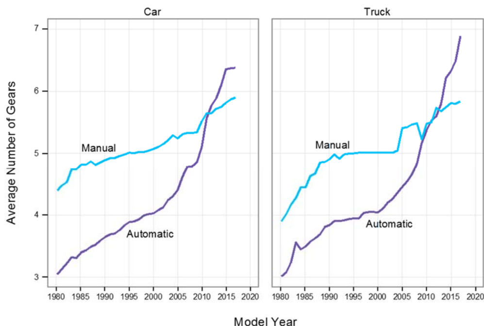
Figure 6-123 - Average Number of Transmission Gears for New Vehicles 253
