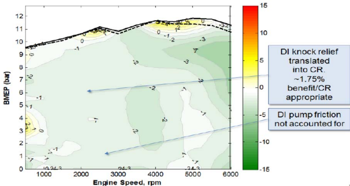
Figure A-4: Comparison of IAV Engine3 Map to IAV Engine2 Map
