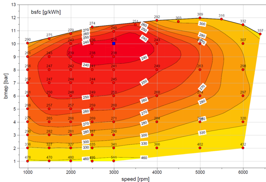
Figure 6-77 - Engine efficiency map for eng7a
