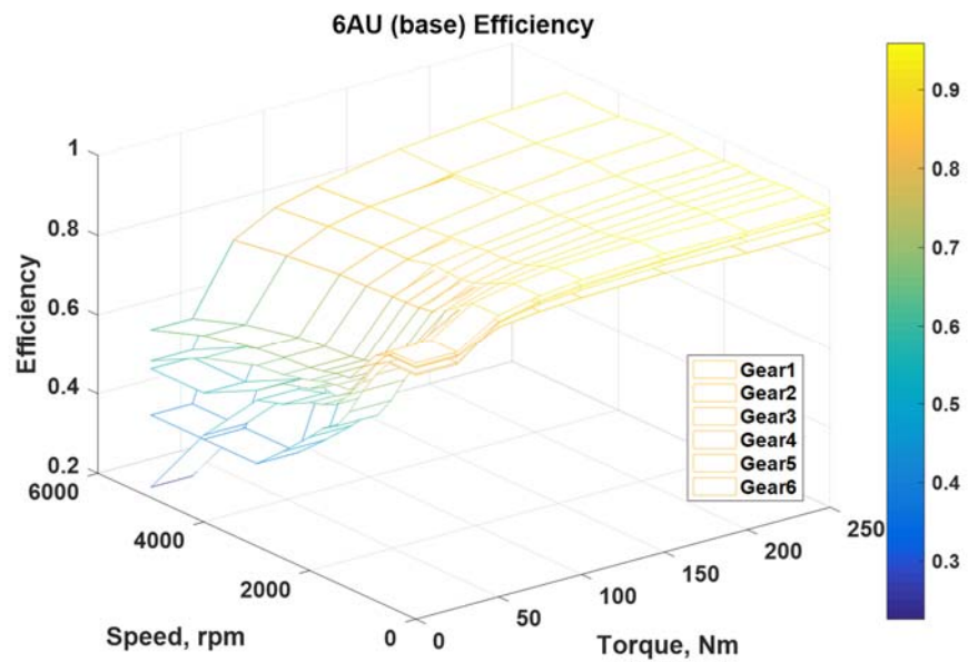
Figure 6-127 - Efficiency map - Base 6-speed automatic level 1
