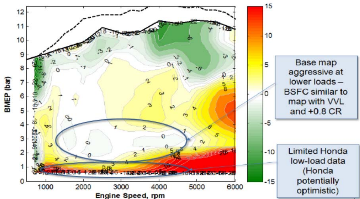
Figure A-2: Comparison of NHTSA Base Engine Map to Honda Accord 2.4L Engine
