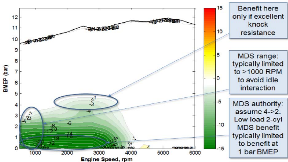
Figure A-6: Comparison of IAV Engine4 Map to IAV Engine3 Map
