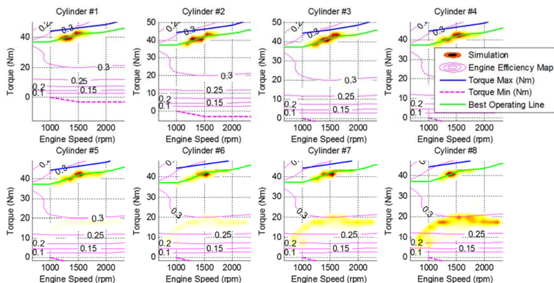
Figure 6-65 - Example of 8-cylinder Energy Density of cylinders operating points in optimum load
