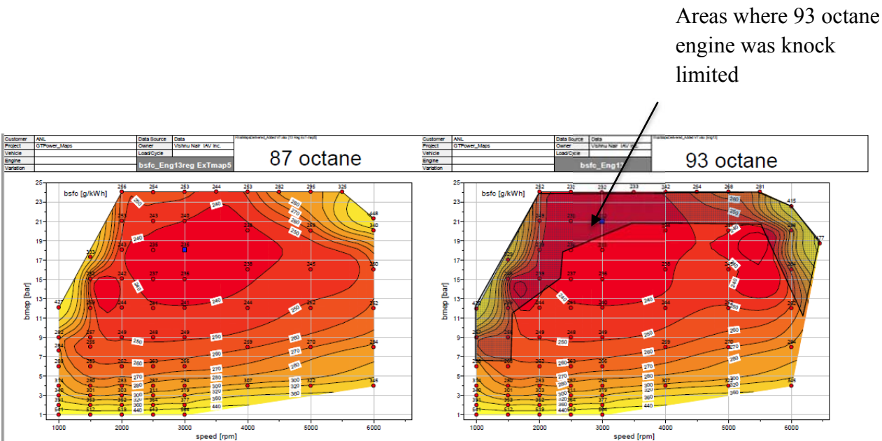
Figure 6-88 - BSFC of 93 (right) versus 87 (left) octane fuel for eng13
