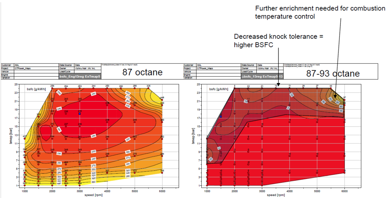
Figure 6-89 - Delta BSFC of 93 (right) versus 87 (left) octane fuel for eng13
