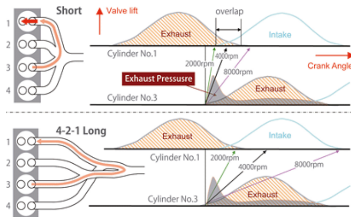
Figure 6-43 - Mazda SkyActiv 4-2-1 exhaust system to mitigate knocking by reducing residual gas. 197
