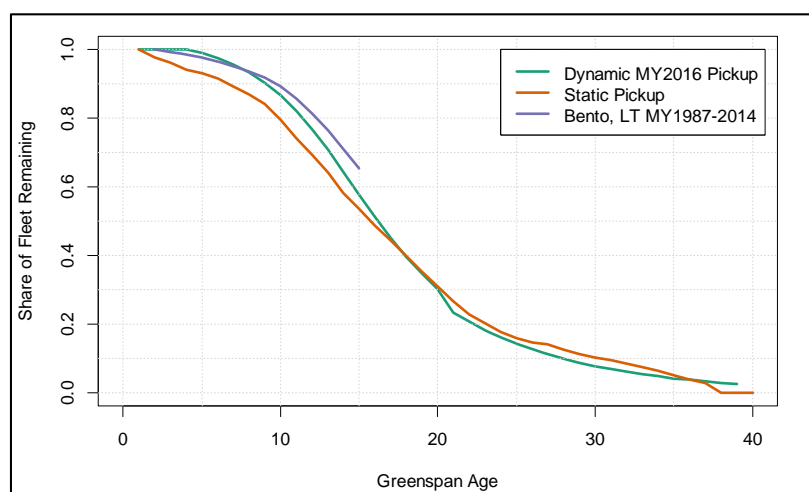
Figure 8-37 - Comparing Different Pickup Scrappage Models
