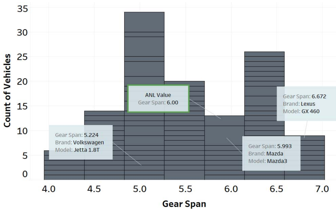
Figure 6-31 - Example of vehicle attribute analysis for gear span of 6AU transmission
