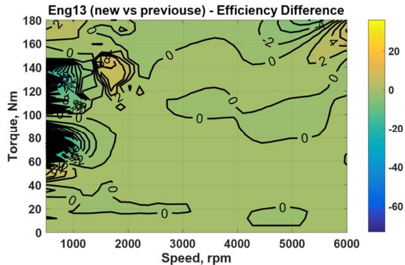
Figure 6-90 - Engine efficiency difference in percent for 93- vs. 87-octane fuel for engine 13
