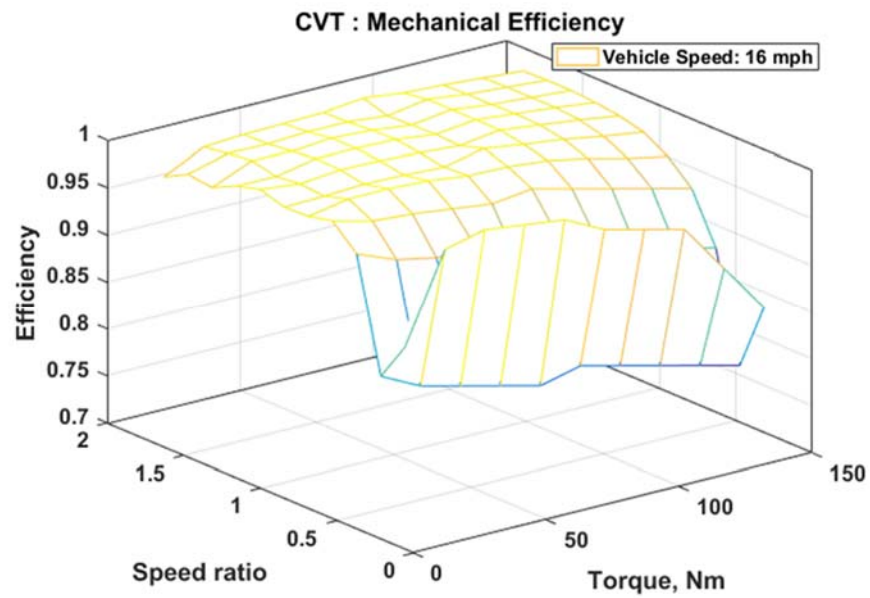
Figure 6-140 - Mechanical efficiency map of CVT level 1 at 16 mph
