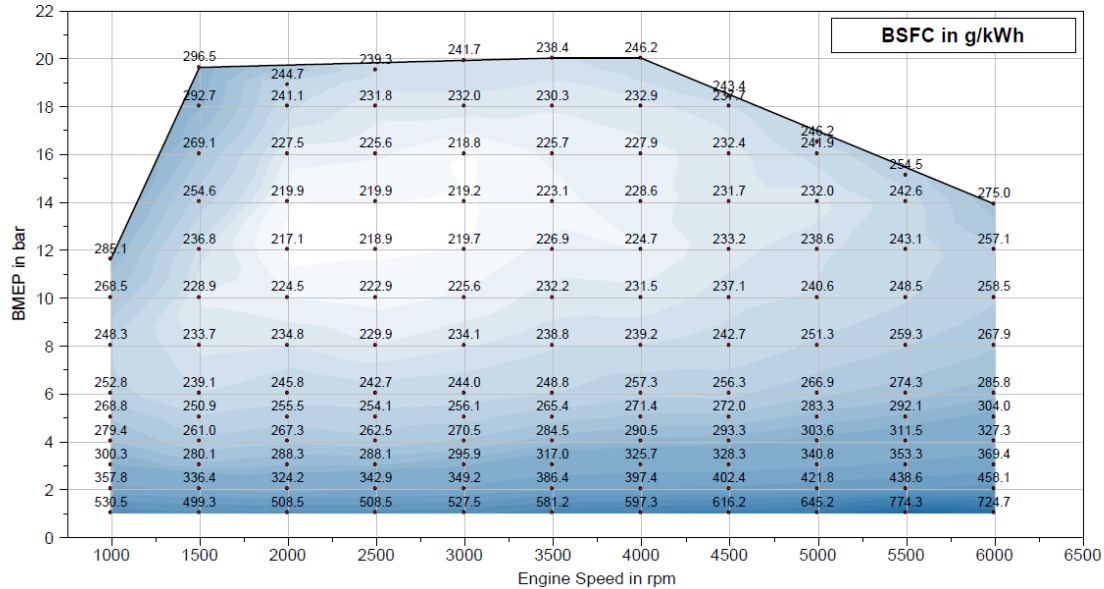
Figure 6-115 - IAV ENGINE 23b's BSFC MAP
