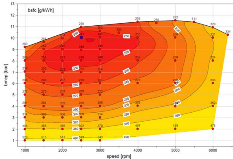
Figure 6-73 - Engine efficiency map for eng5b
