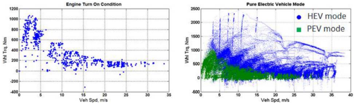
Figure 6-24 - Cycles Wheel Torque Vs Vehicle Speed, 2014 Jetta HEV Based on Test Cycles (data source APRF)
