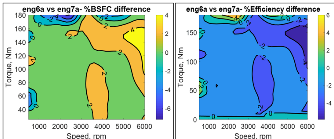
Figure 6-78 - Incremental BSFC and thermal efficiency difference between eng6a versus eng7a
