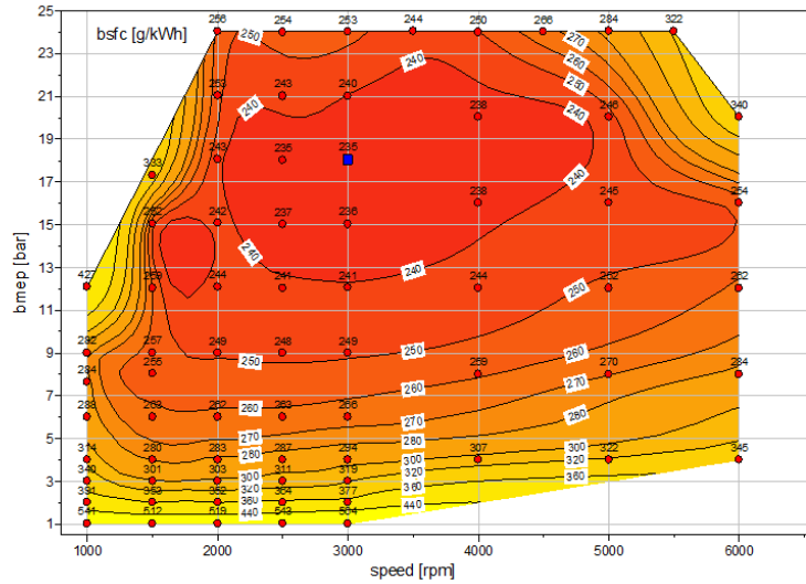
Figure 6-91 - Engine efficiency map for eng14.
