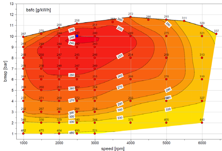
Figure 6-75 - Engine Efficiency Map for eng6a
