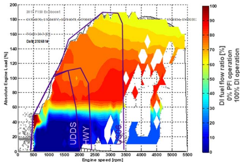
Figure 6-38 - DI and PFI usage map as function of engine speed and load for a 2017 Ford F150 3.5L Ecoboost 183
