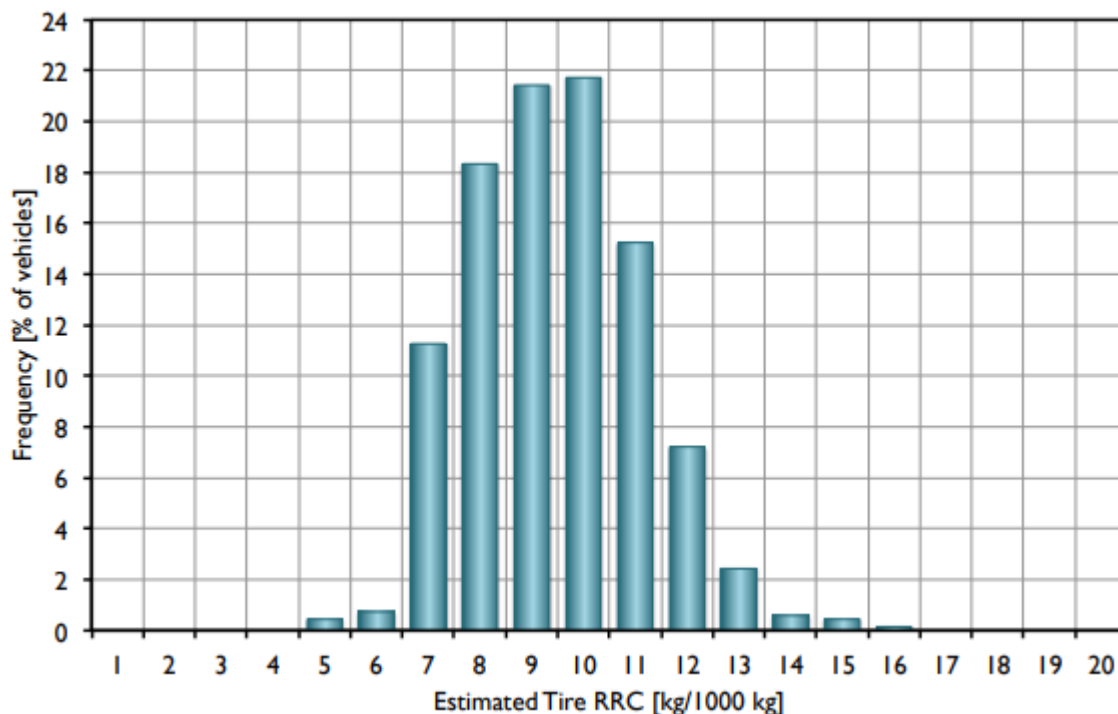
Figure 6-176 - CONTROLTEC distribution of estimated tire RRC for all vehicles 405
