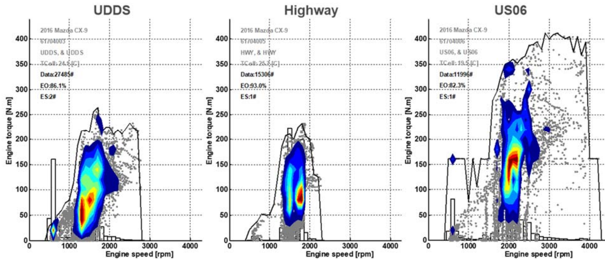
Figure 6-42 - Engine operating Area on certification cycles of 2016 Mazda CX-9 benchmarked by NHTSA 196
