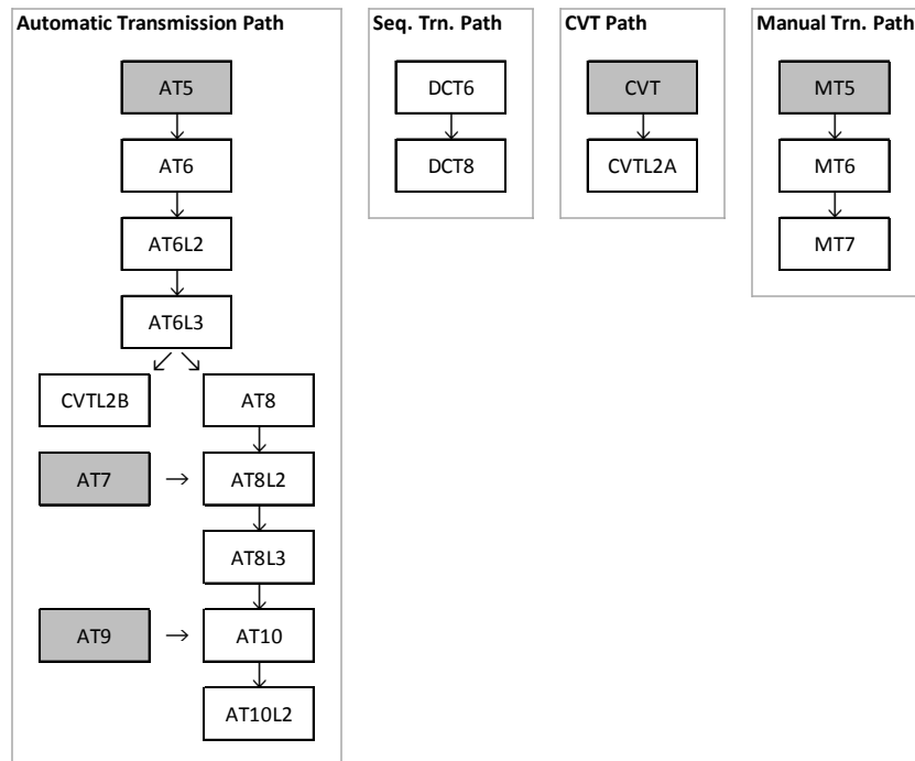
Figure 6-182 - Transmission Paths
