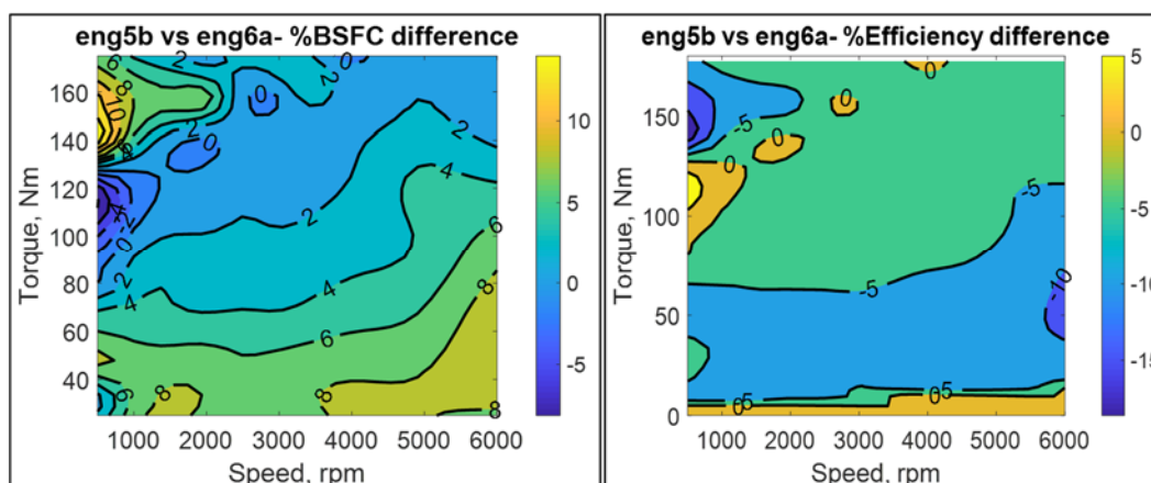
Figure 6-76 - incremental BSFC and thermal efficiency difference between eng05b versus eng6a
