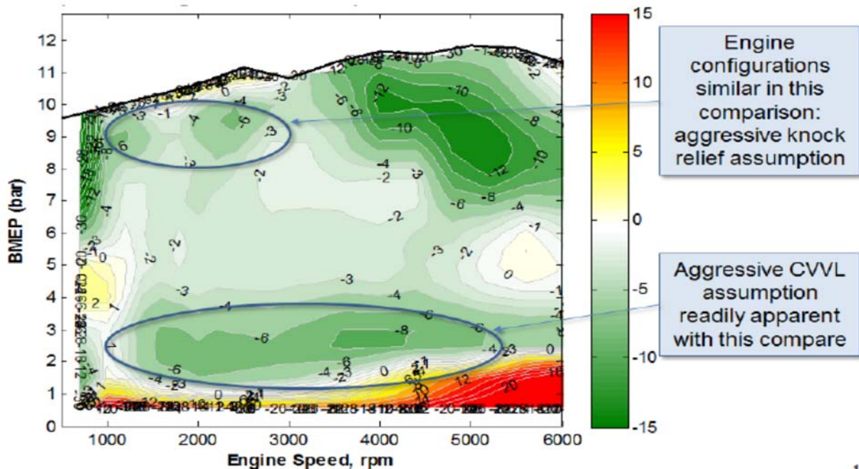
Figure A-5: Comparison of IAV Engine3 Map to Honda Accord 2.4L Engine
