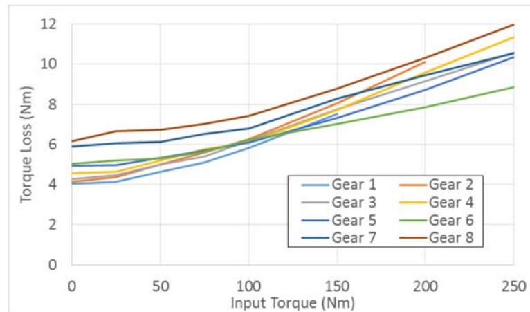
Figure 6-121 - Average Torque Losses in Each Gear for an Eight-Speed 845RE Transmission 248
