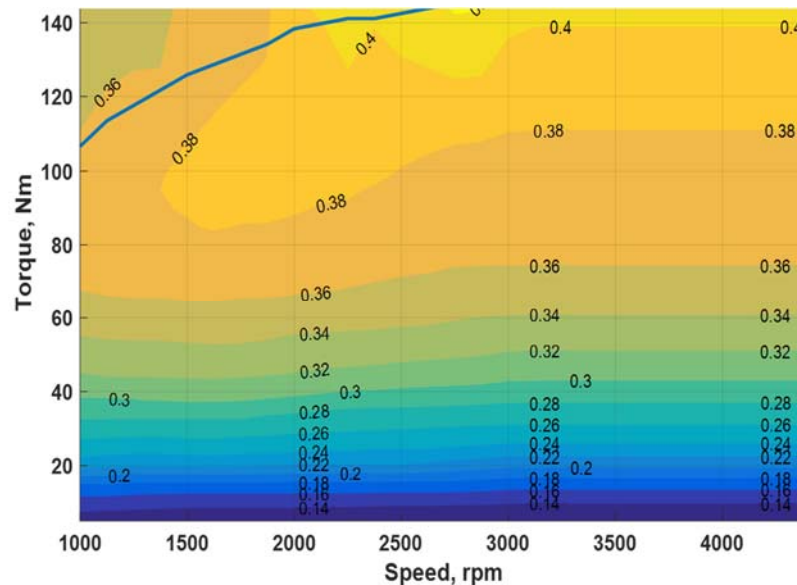
Figure 6-110 - Engine Efficiency Map for eng26
