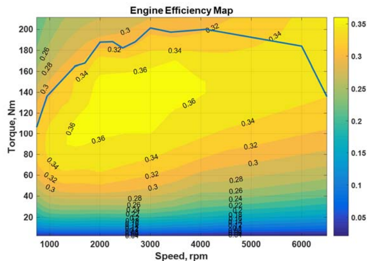
Figure 6-41 - BTE for a Representative MY 2010 2.4L NA PFI tested by EPA. 194, 195
