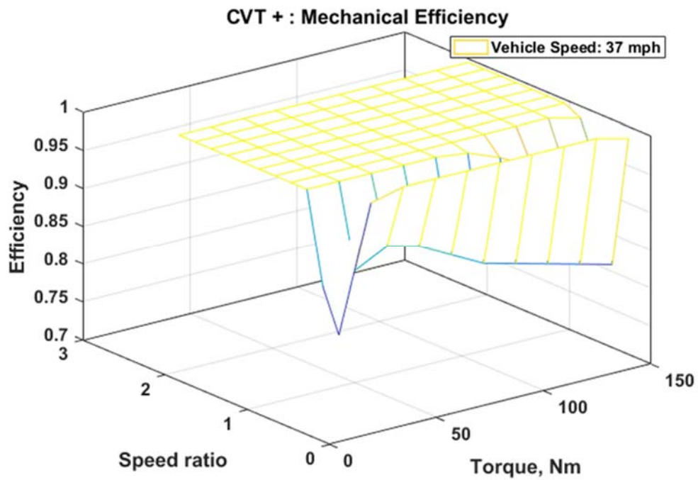
Figure 6-146 - Mechanical Efficiency map of CVT level 2 at 37 mph
