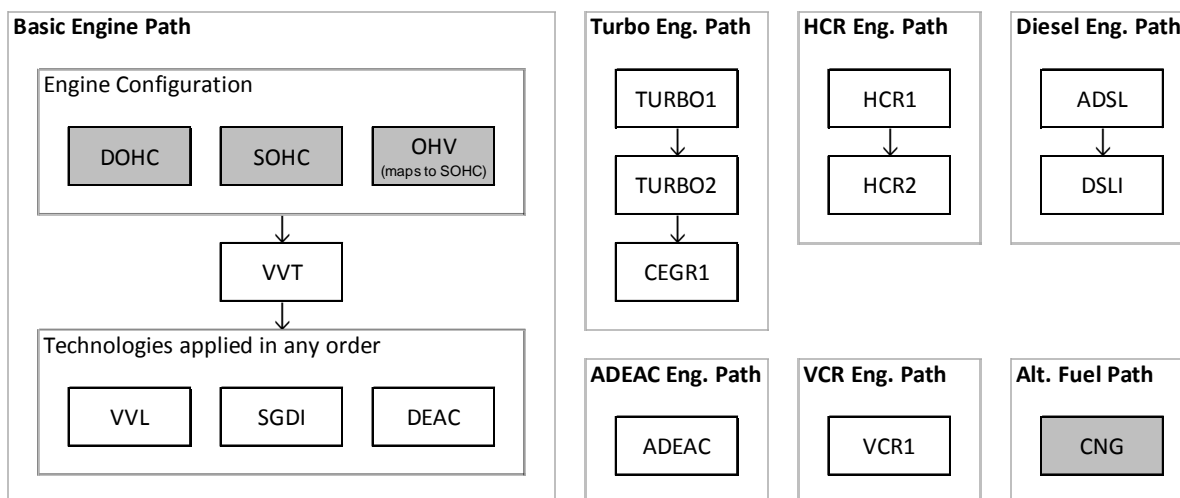
Figure 6-181 - Engine Paths
