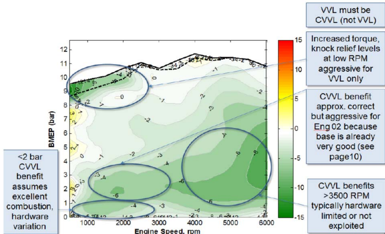
Figure A-3: Comparison of IAV Gasoline Engine2 Map to NHTSA Base Engine Map
