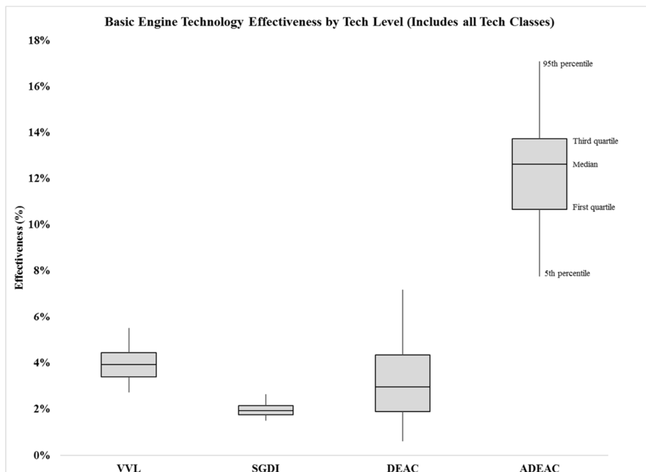
Figure 6-118 shows the effectiveness of engine technologies across different other technologies
