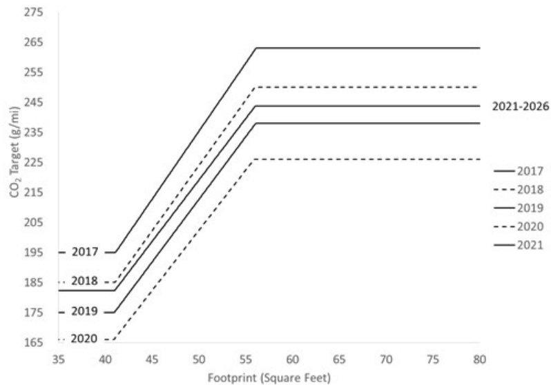
Figure 4-26 - Passenger Car CO 2 Targets 101
