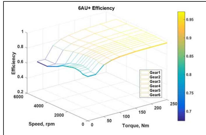
Figure 6-129 - Efficiency map - 6-speed Automatic level 2
