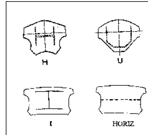
Illustrations of Driver Side Air Bag Tear Patterns
