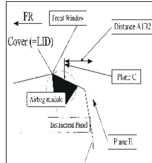
Diagram of Plane C to Plane E for Top-Mounted Air Bags
