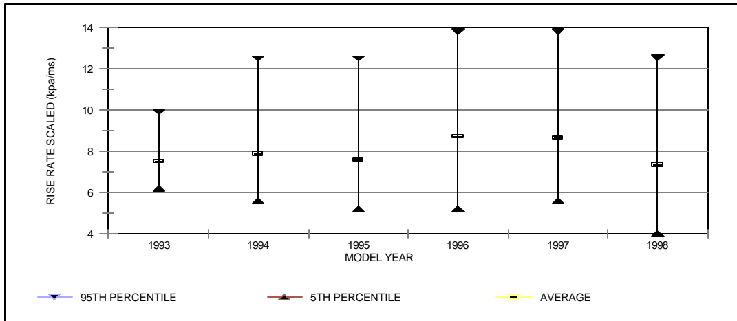
Passenger Side Air Bag: Scaled Rise Rate, 1993-1998
