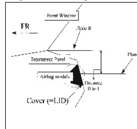
Diagram of Planes B and I for Air Bags Other than Top-Mounted
