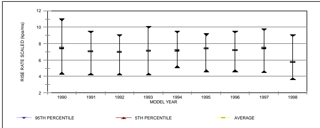
Driver Side Air Bag: Scaled Rise Rate, 1990-1998
