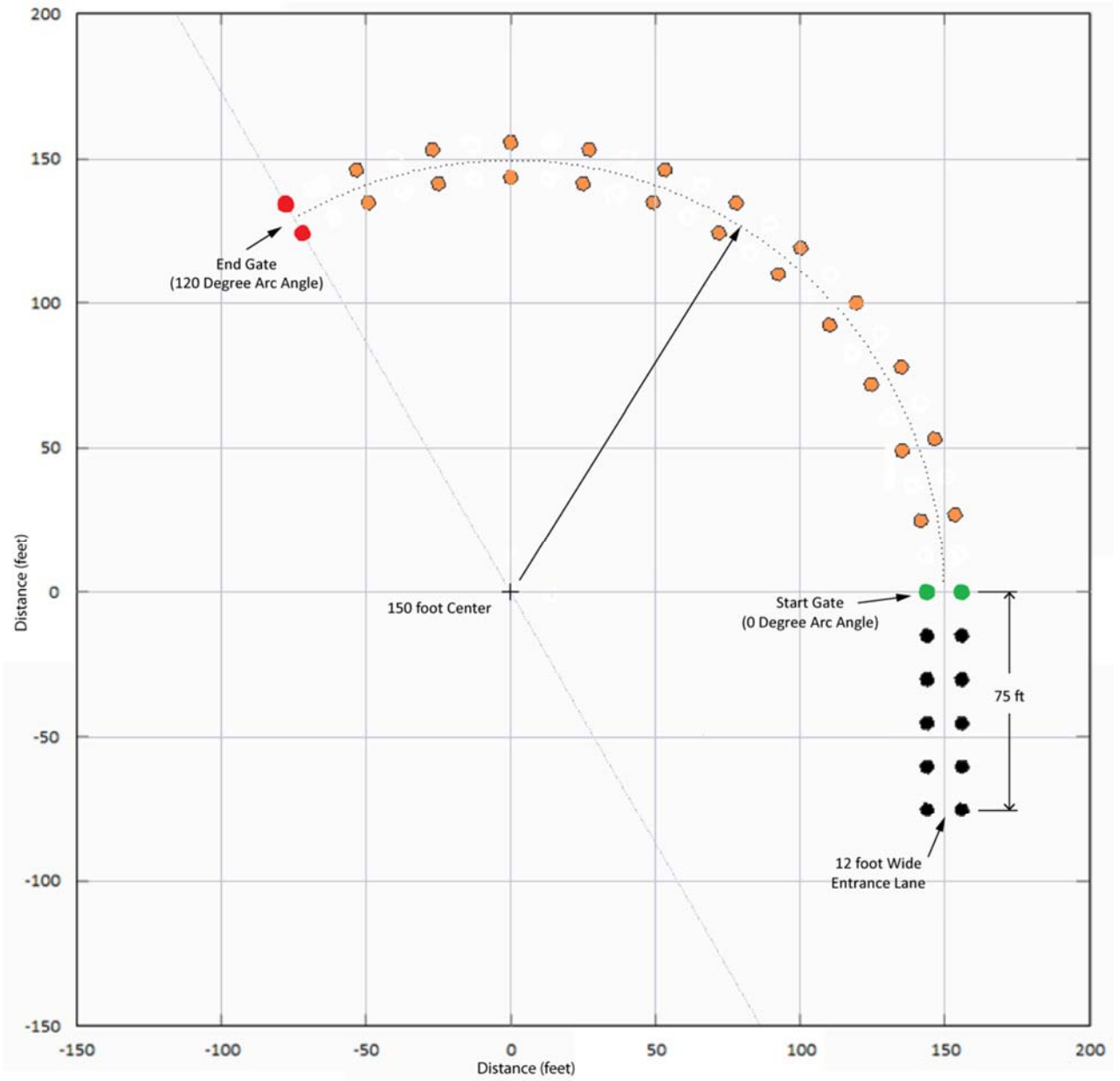
Figure 2 - J-Turn Maneuver Test Course (counter-clockwise)
