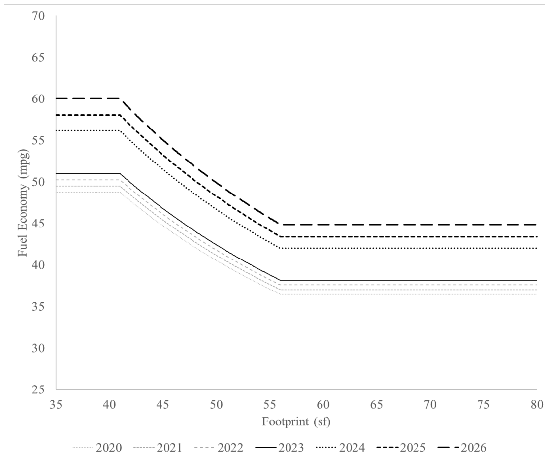
Figure IV-3 – Alternative 1, Passenger Car Fuel Economy, Target Curves
