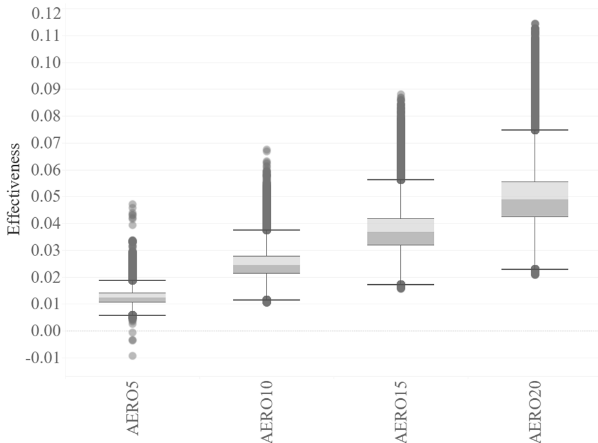
Figure III-15 – AERO Technology Effectiveness 250
