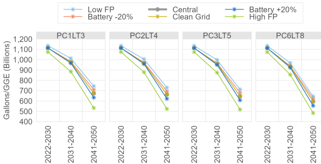
Figure 8-45: Comparison of Fuel Consumption Across Sensitivity Cases in the Action Alternatives
