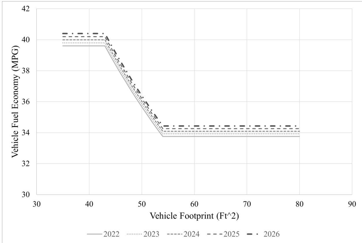
Figure III-9: Alternative 3, Passenger Car Fuel Economy, Target Curves for the MYs 2022-2026 Amendment
