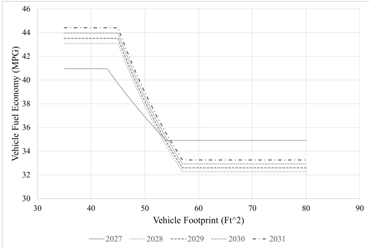
Figure III-15: Alternative 3, Passenger Car Fuel Economy, Target Curves for the MYs 2027-2031 Amendment
