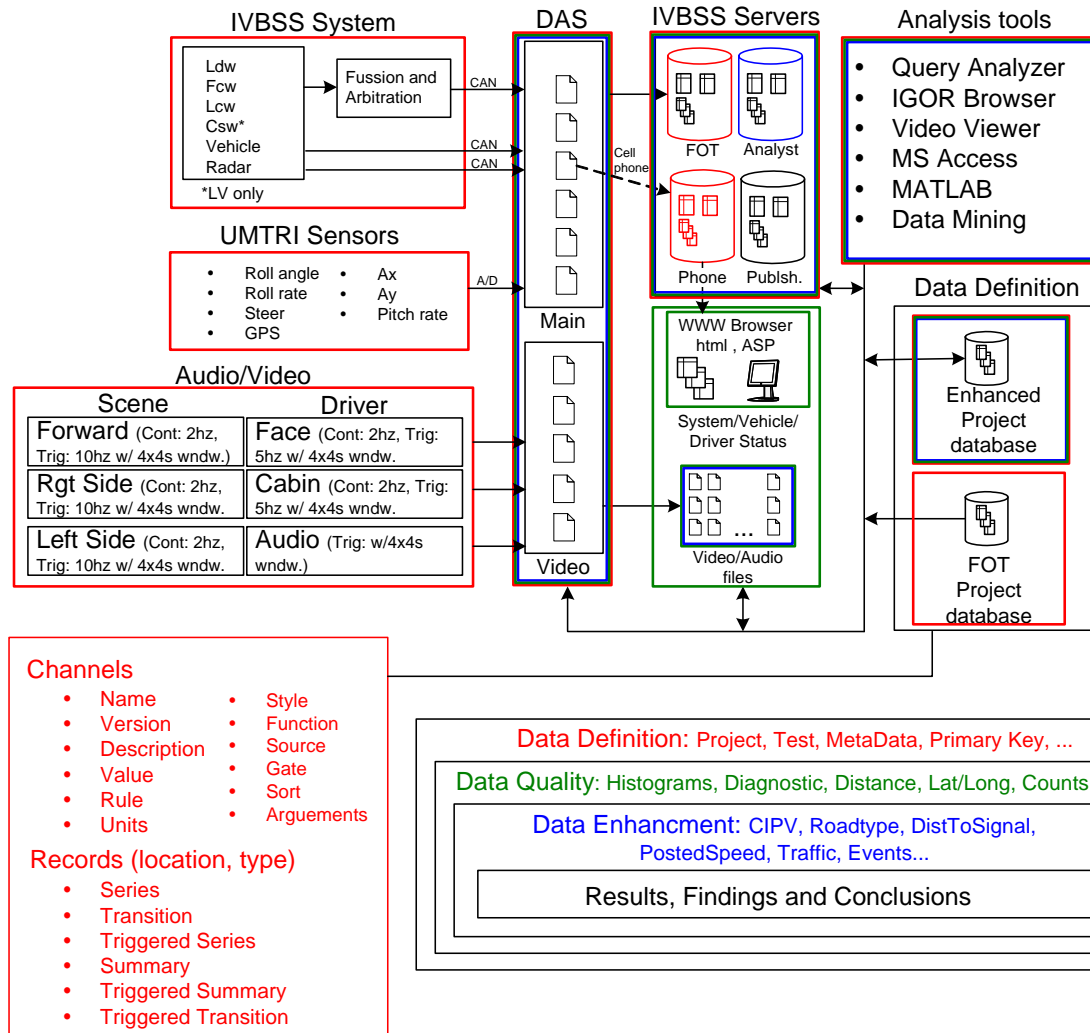
Figure 21. UMTRI data architecture
