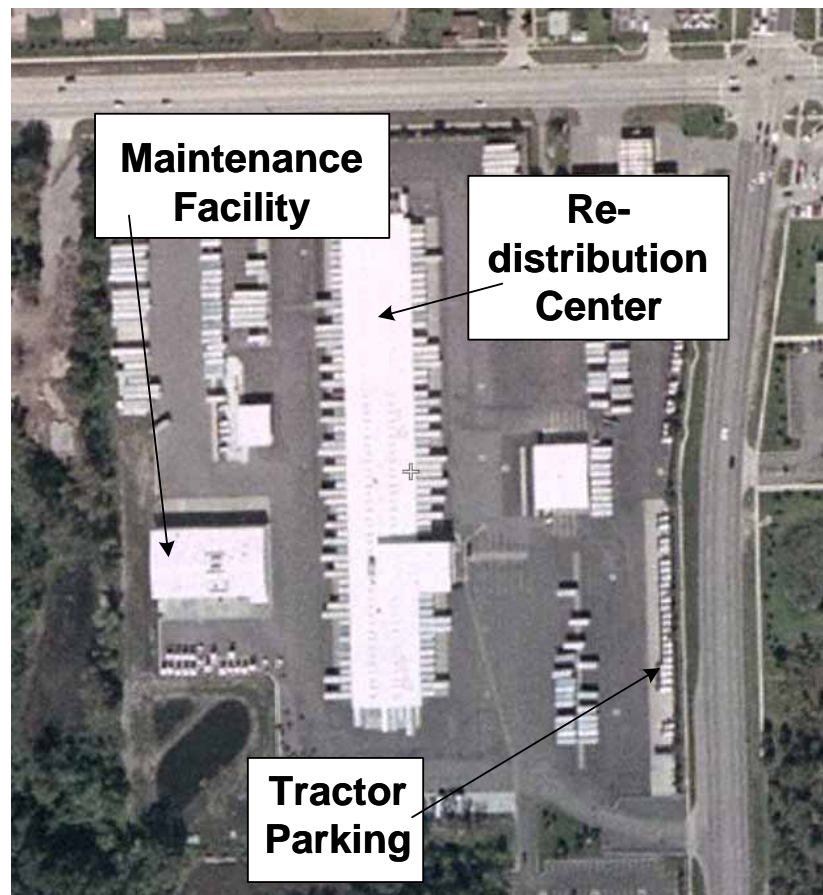
Figure 18. Plan-view of the Con-way facility at Romulus, Michigan
