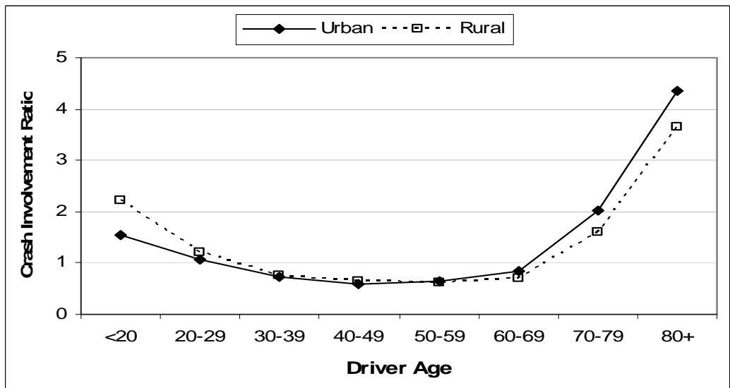
Figure 10. Two-vehicle fatal CIRs on urban versus rural roadways.
