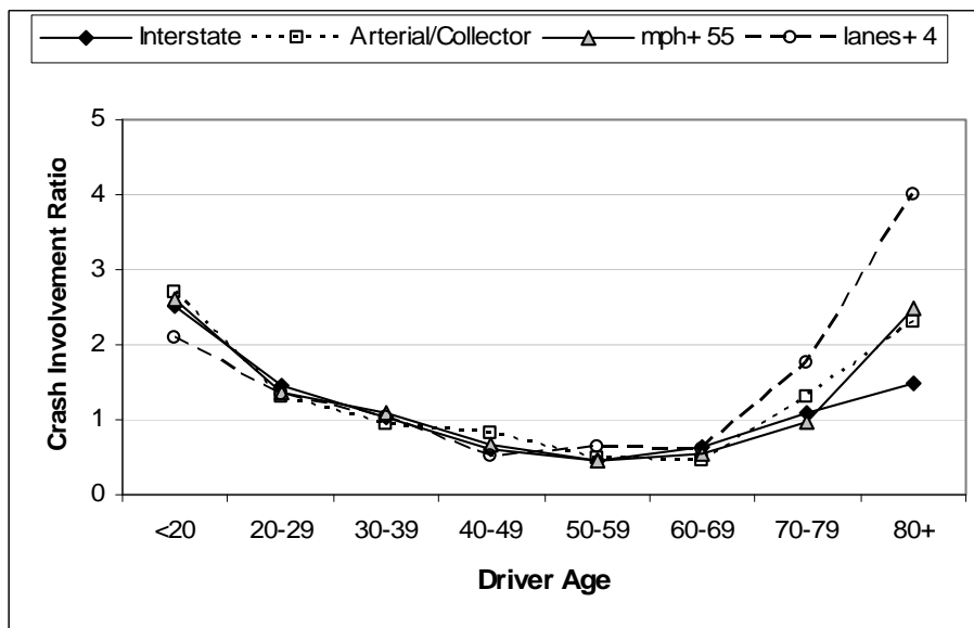
Figure 16. Two-vehicle fatal CIRs for changing lanes or merging on various types of roadways.
