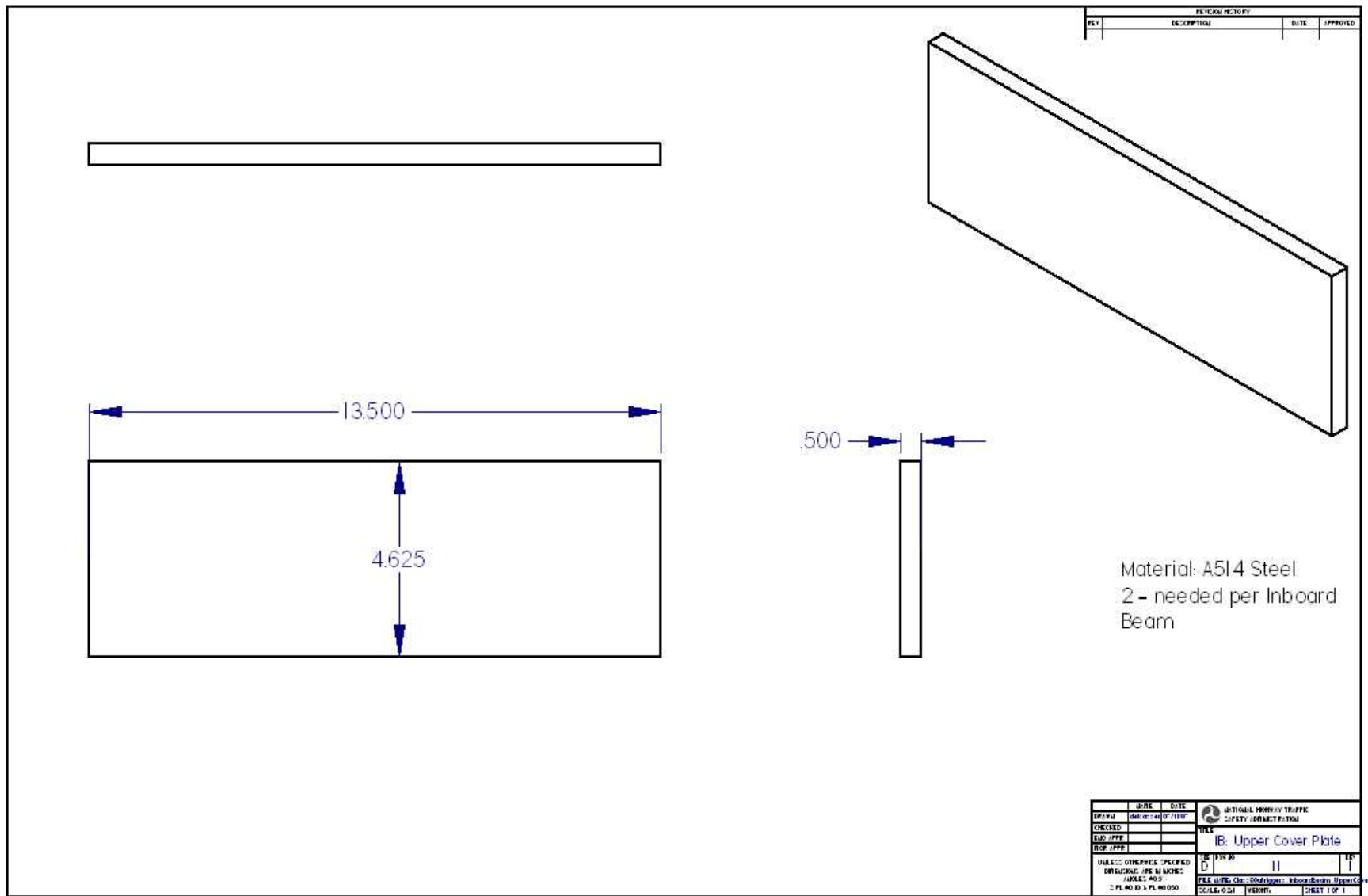
Figure A.17: Draft of Upper Cover Plate for the Inboard Beam.
