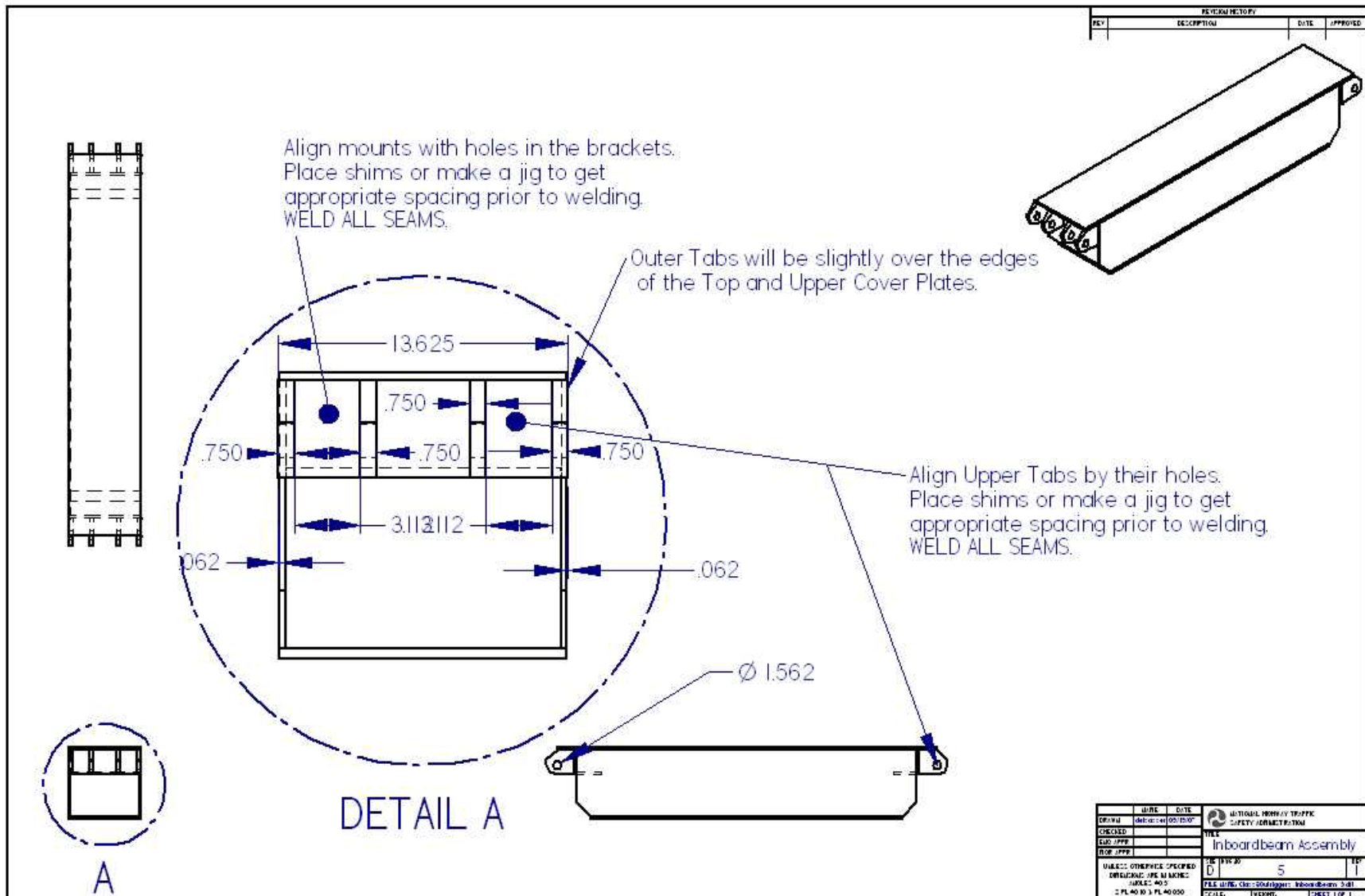
Figure 4.13: Sixth step; tack weld in place the Upper Tabs using the Aluminum Hinges and shims as jigs to assure free play tolerances. All seems were welded.
