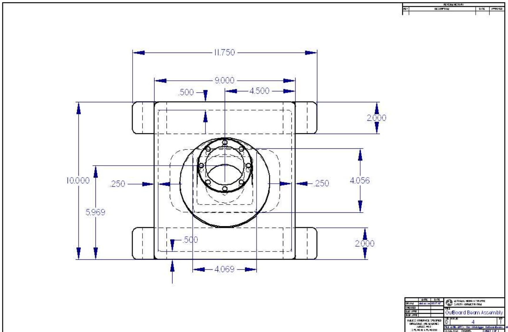
Figure A.11: End view (Axle and End Plate placement) draft of the Outboard Beam assembly.
