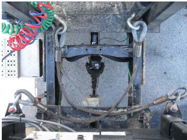
Figure B.3. Anti-jackknife cables
