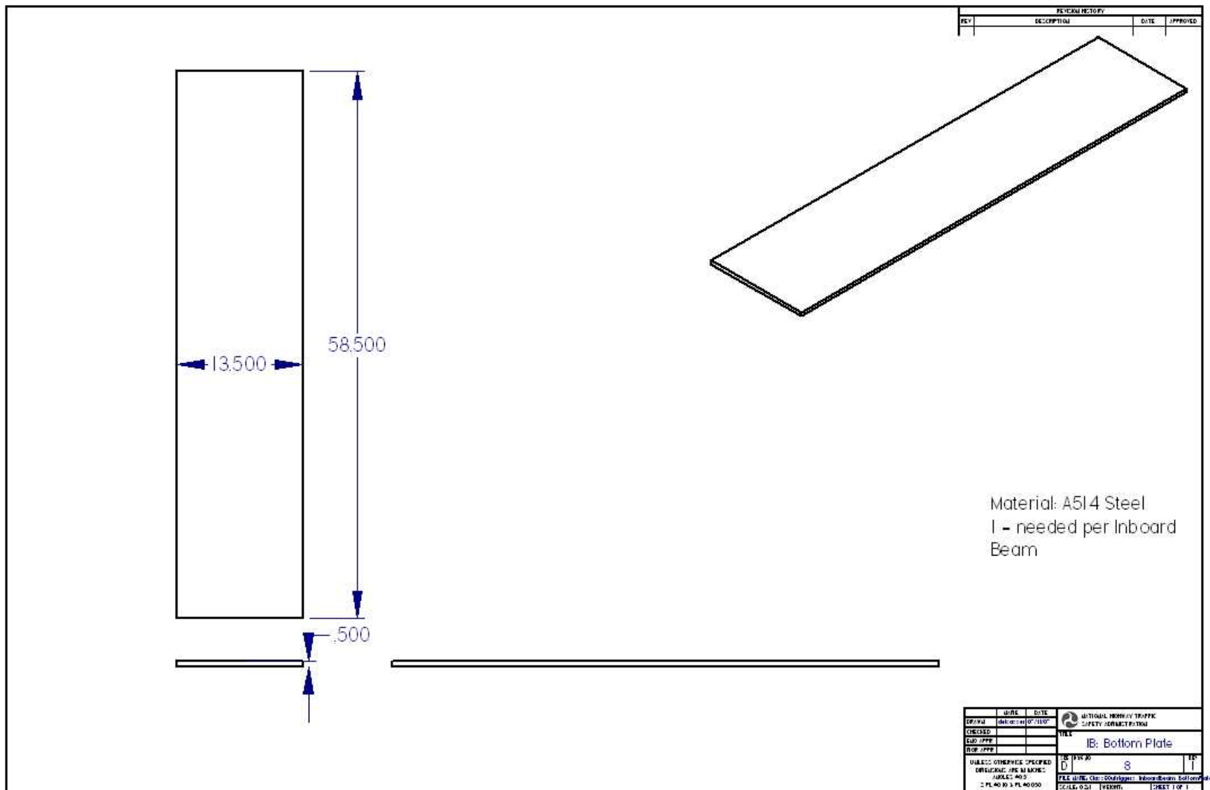
Figure A.14: Draft of Bottom Plate for the Inboard Beam.
